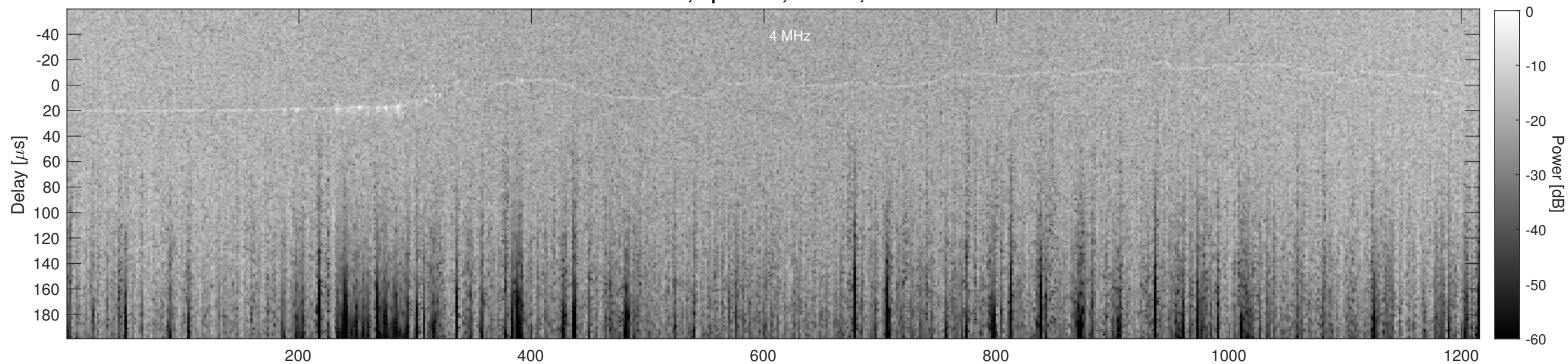
Orbit 13569, Cluttergram
