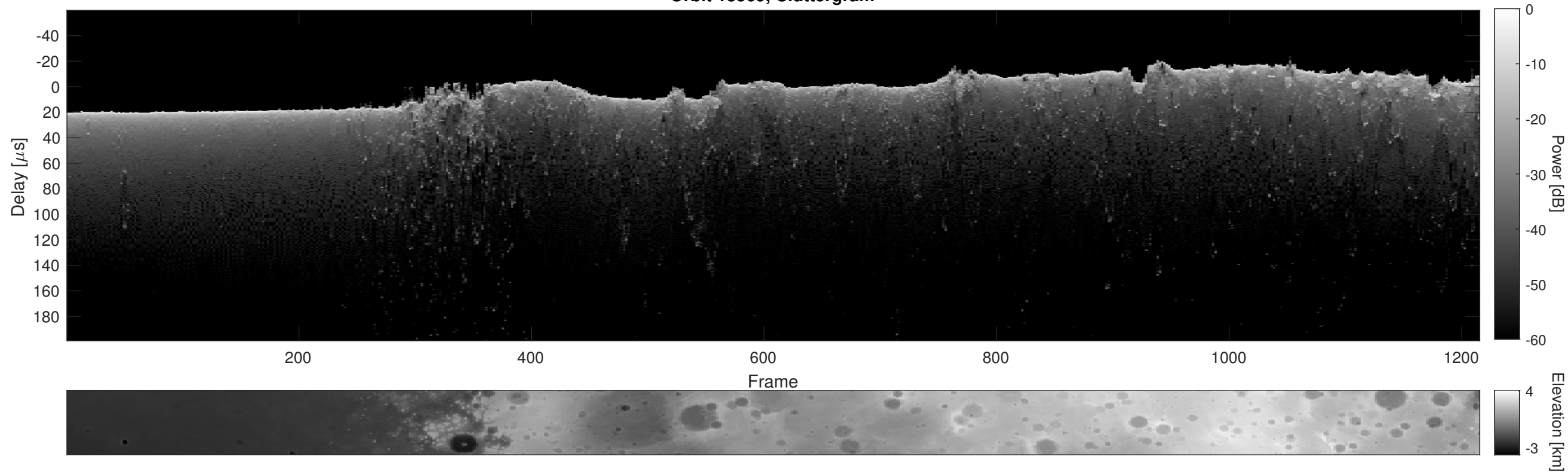
Orbit 13569, Cluttergram
