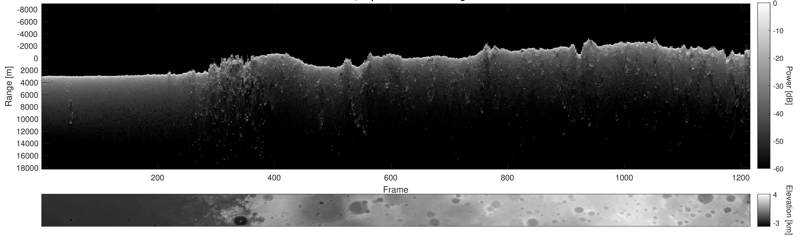
Orbit 13569, Depth-Corrected Cluttergram
