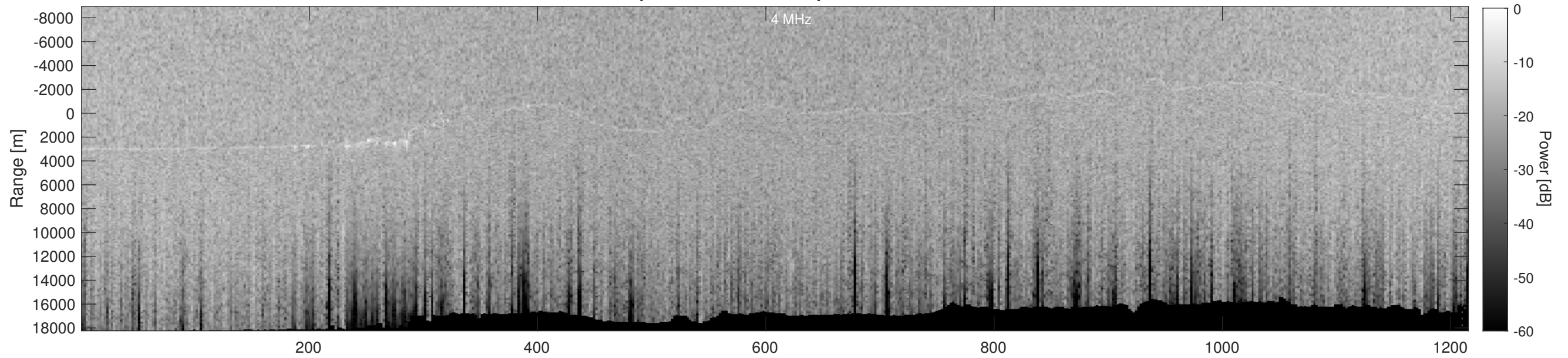
Orbit 13569, Depth-Corrected Cluttergram
