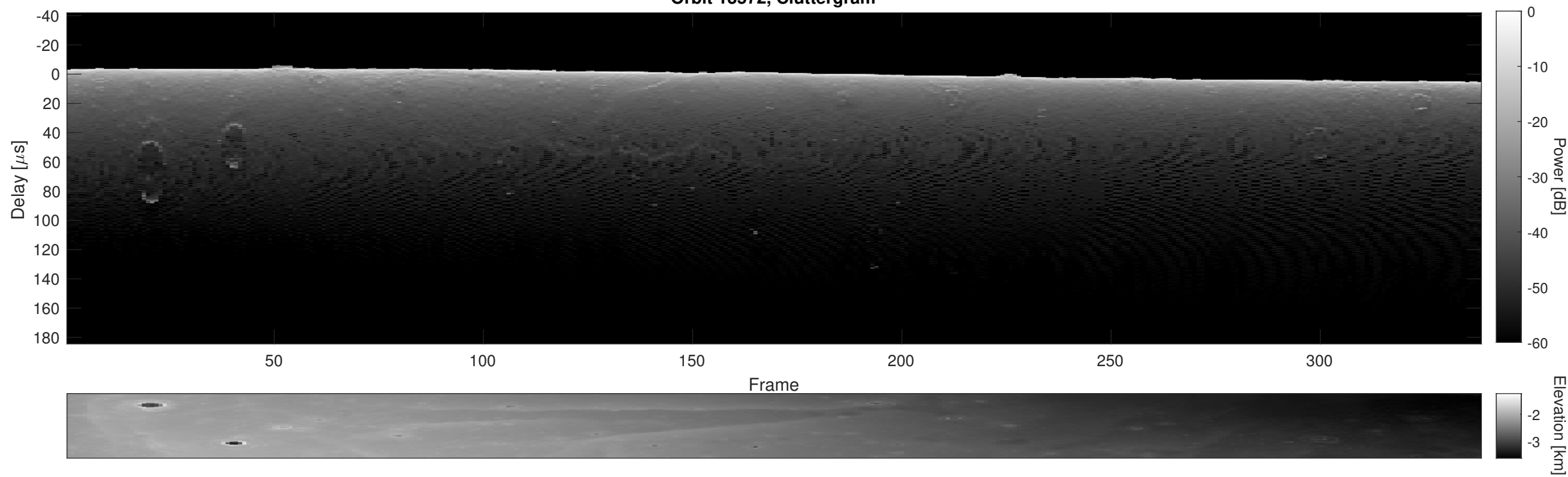
Orbit 13572, Cluttergram
