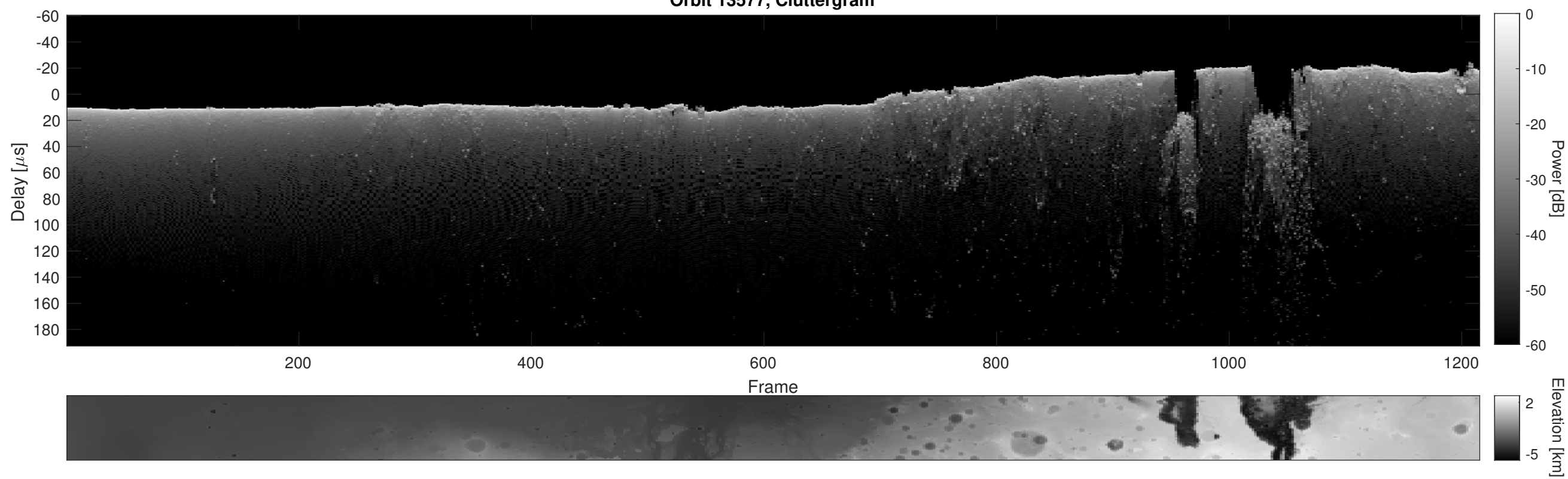
Orbit 13577, Cluttergram
