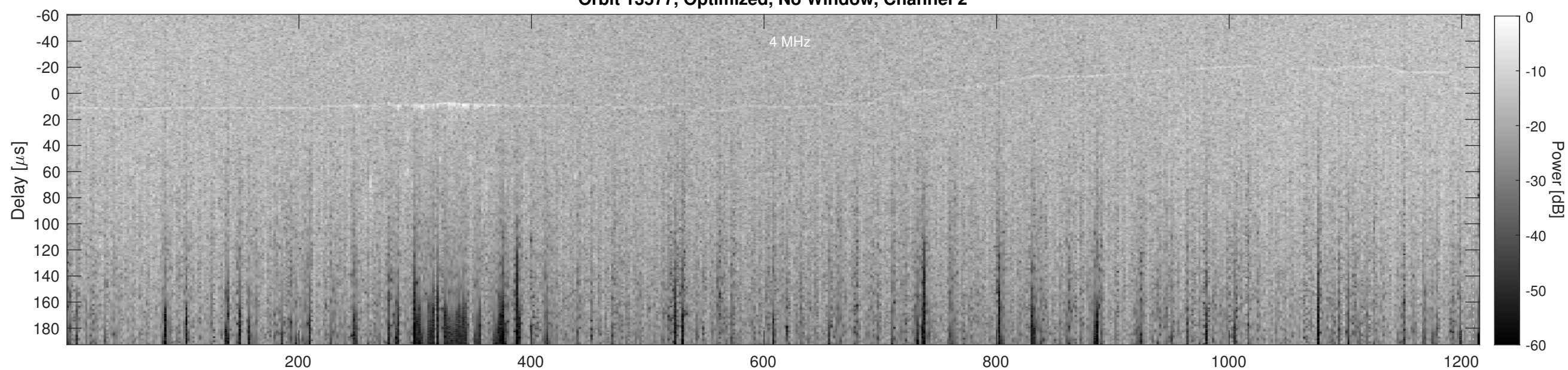
Orbit 13577, Cluttergram
