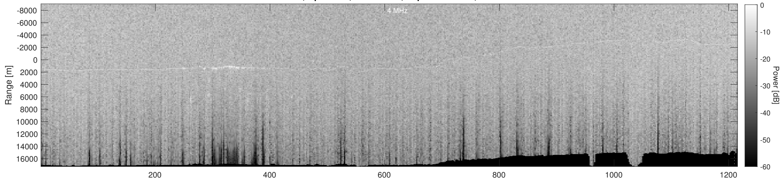
Orbit 13577, Depth-Corrected Cluttergram
