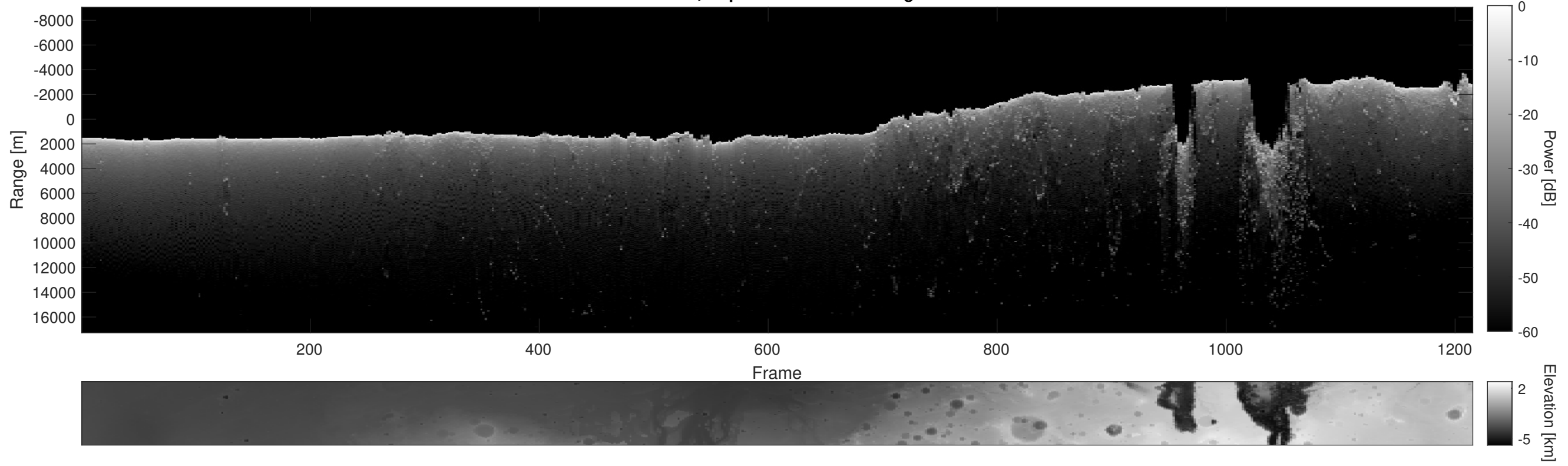
Orbit 13577, Depth-Corrected Cluttergram
