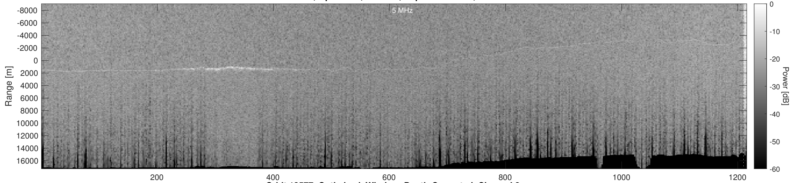
Orbit 13577, Optimized, Window, Depth-Corrected, Channel 2
