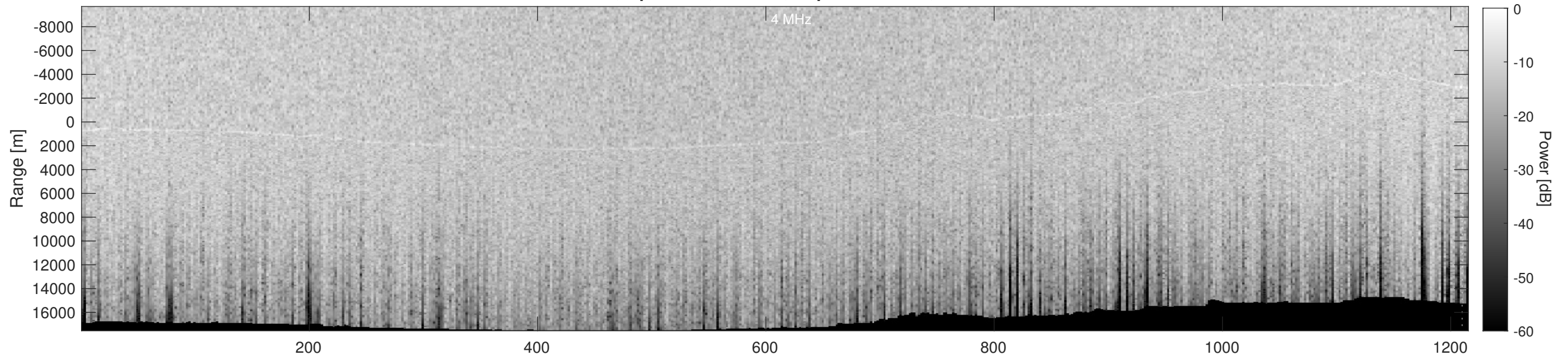
Orbit 13579, Depth-Corrected Cluttergram
