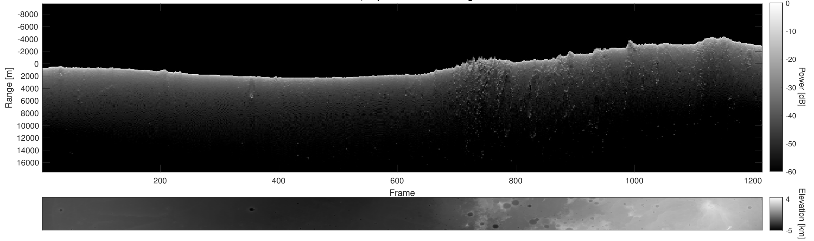
Orbit 13579, Depth-Corrected Cluttergram
