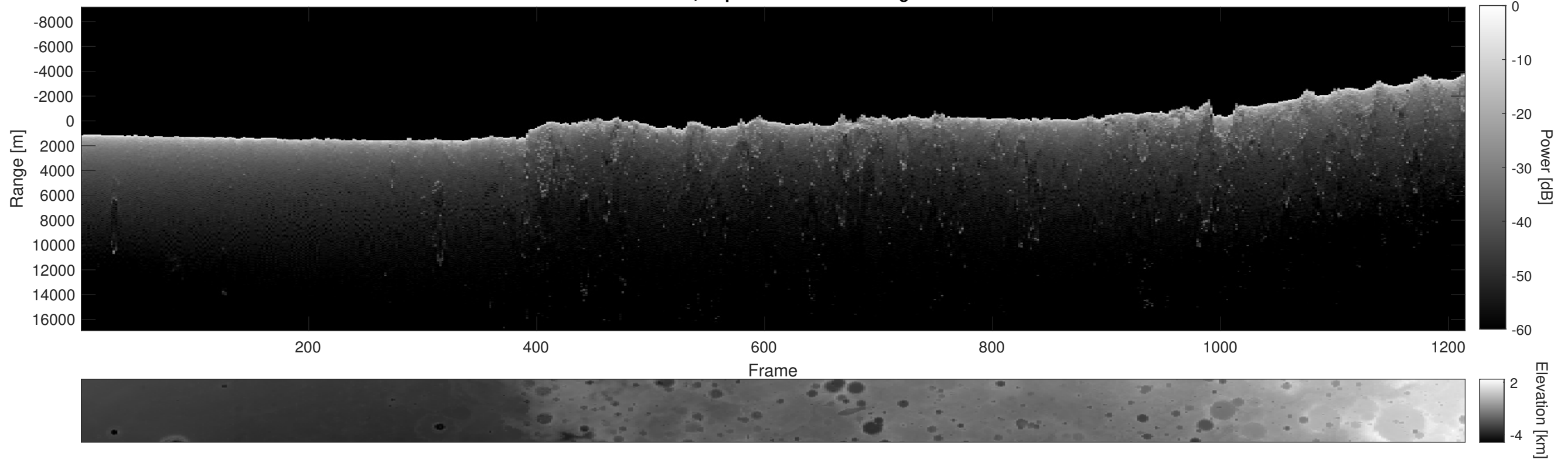
Orbit 13580, Depth-Corrected Cluttergram
