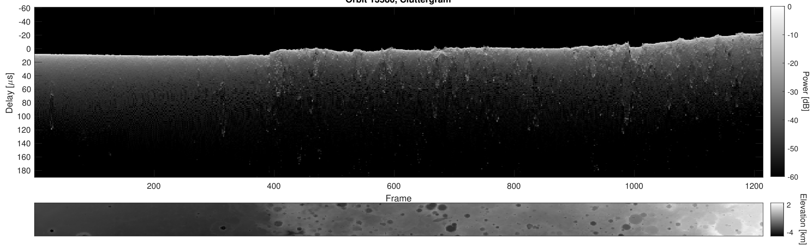
Orbit 13580, Cluttergram
