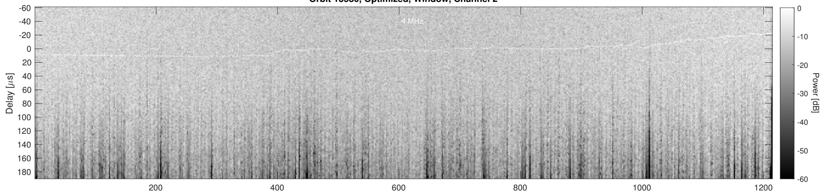
Orbit 13580, Cluttergram
