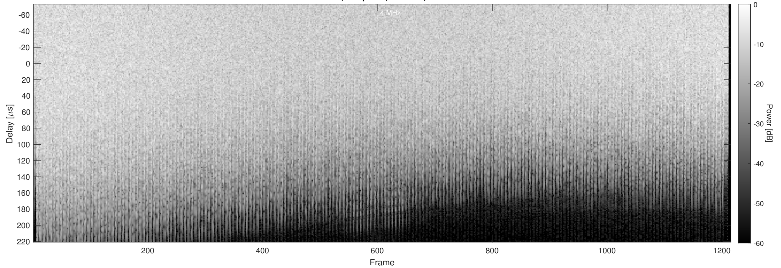
Orbit 13581, Chapman, Window, Channel 2
