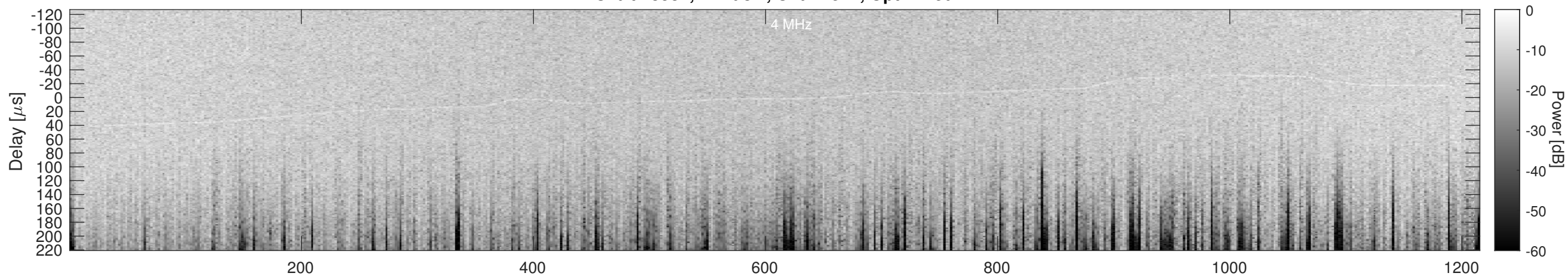
Orbit 13581, Cluttergram
