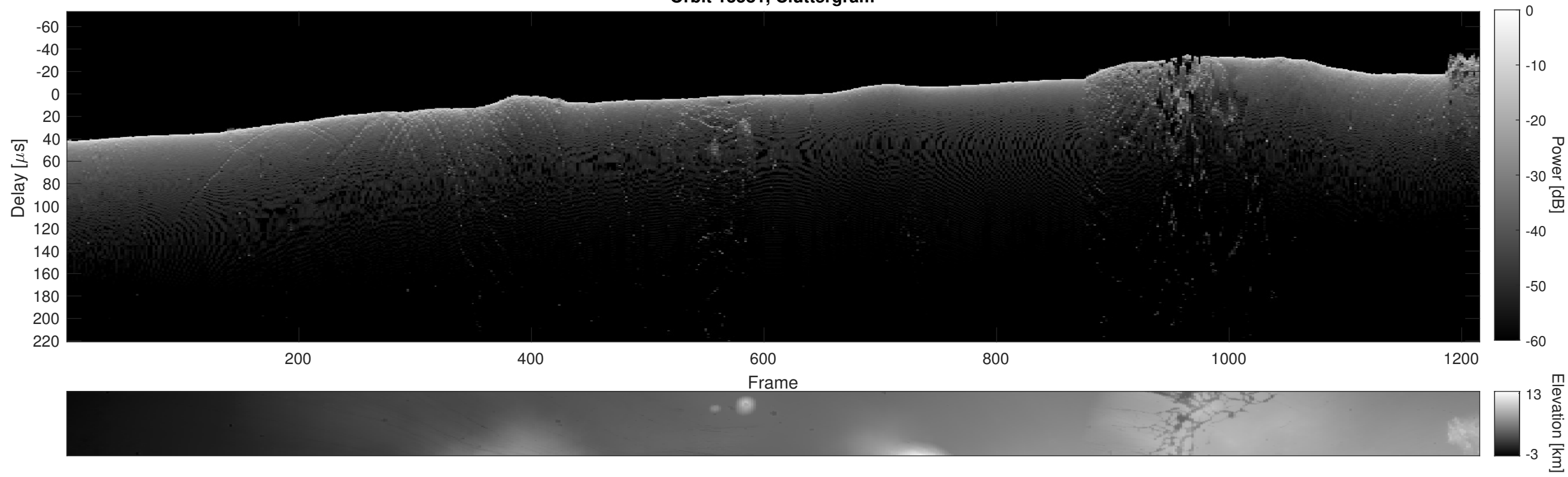
Orbit 13581, Cluttergram
