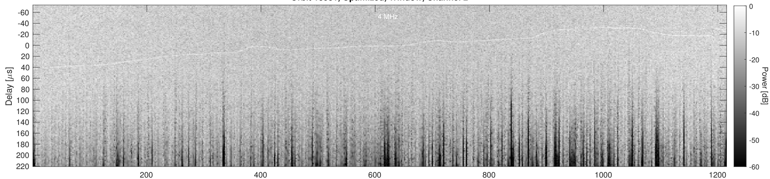
Orbit 13581, Cluttergram
