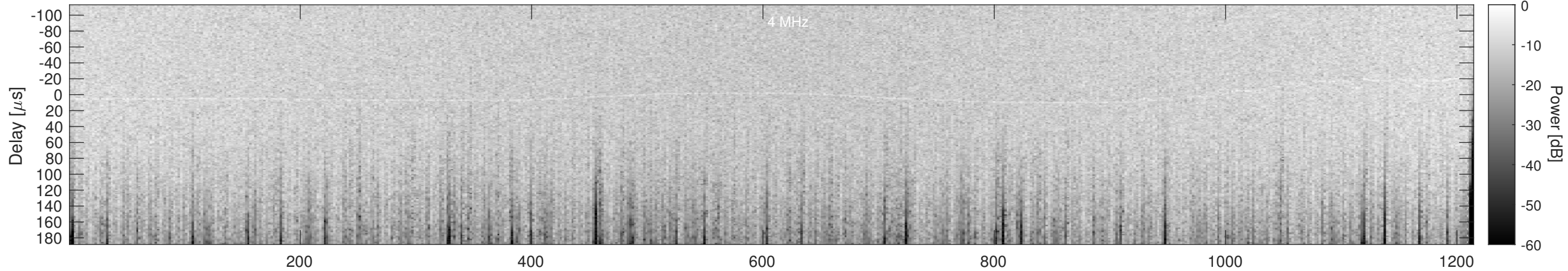
Orbit 13582, Cluttergram
