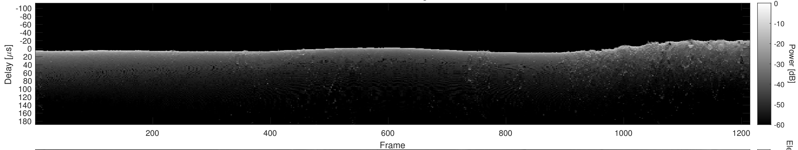
Orbit 13582, Cluttergram
