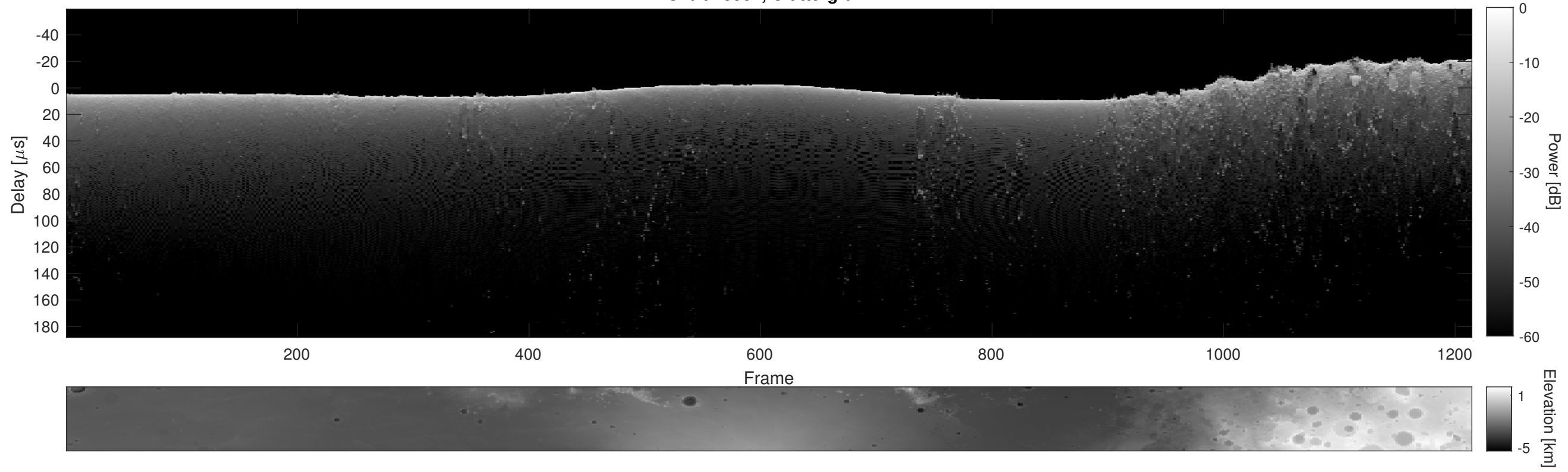
Orbit 13582, Cluttergram
