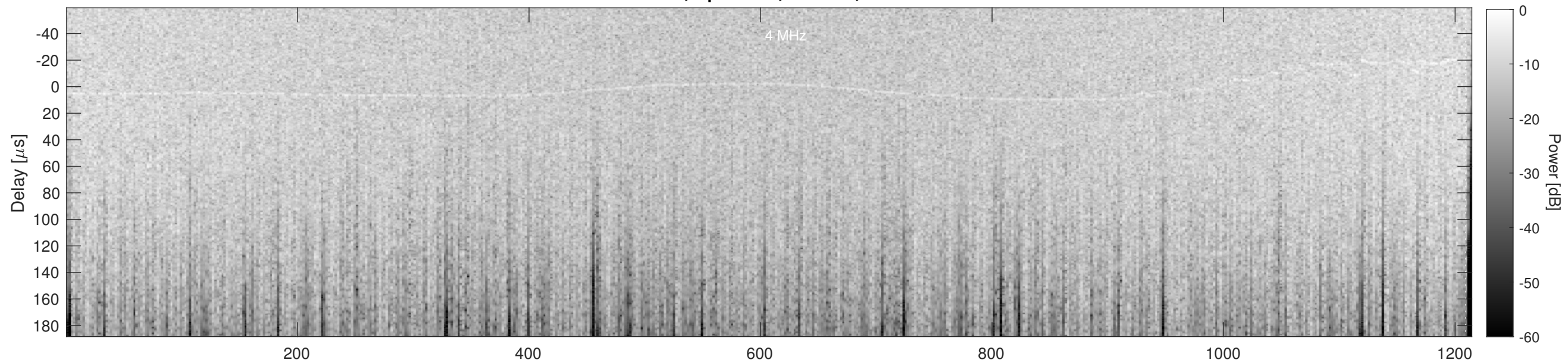
Orbit 13582, Cluttergram
