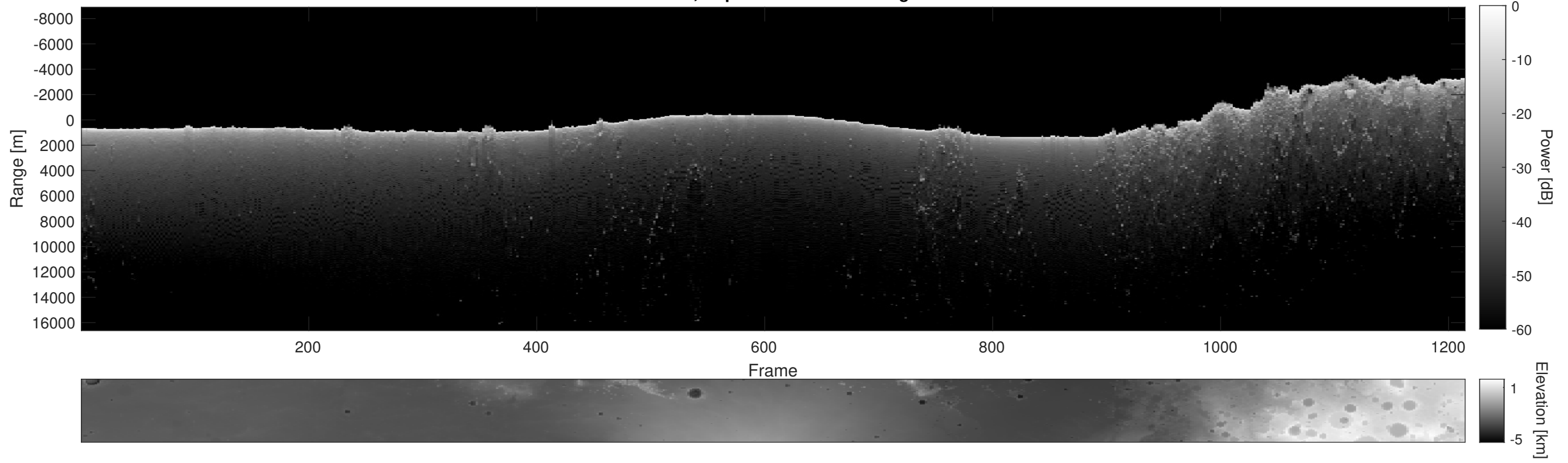
Orbit 13582, Depth-Corrected Cluttergram
