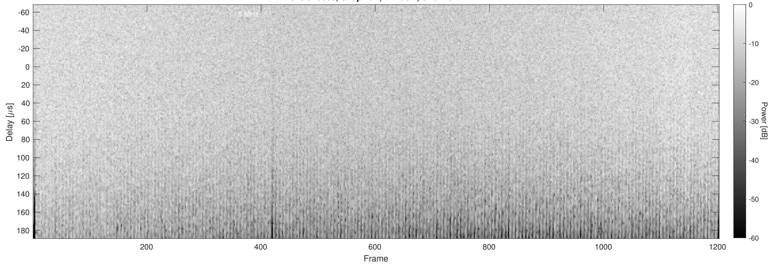
Orbit 13585, Chapman, Window, Channel 2
