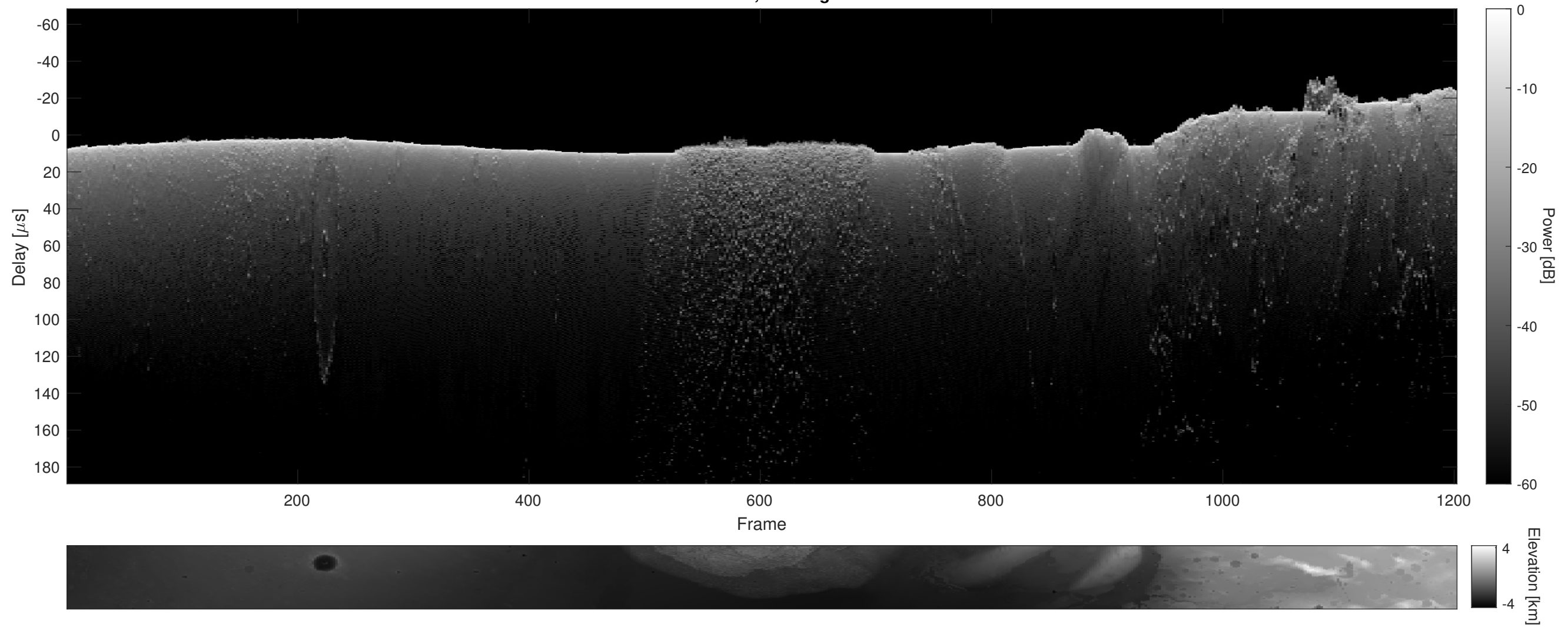
Orbit 13585, Cluttergram
