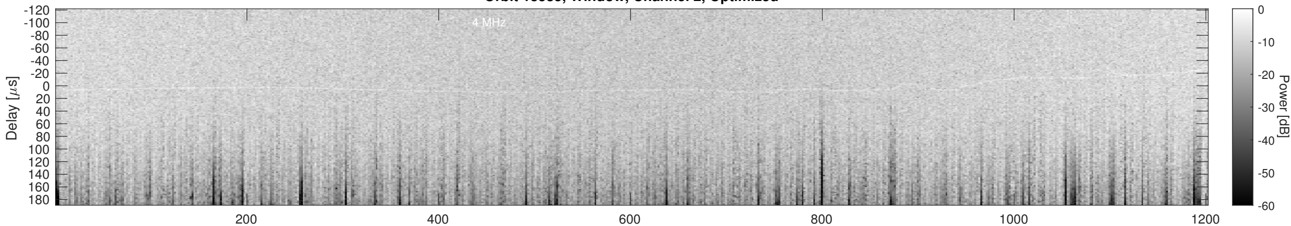
Orbit 13585, Cluttergram
