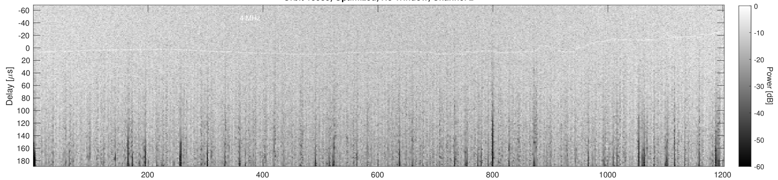
Orbit 13585, Cluttergram
