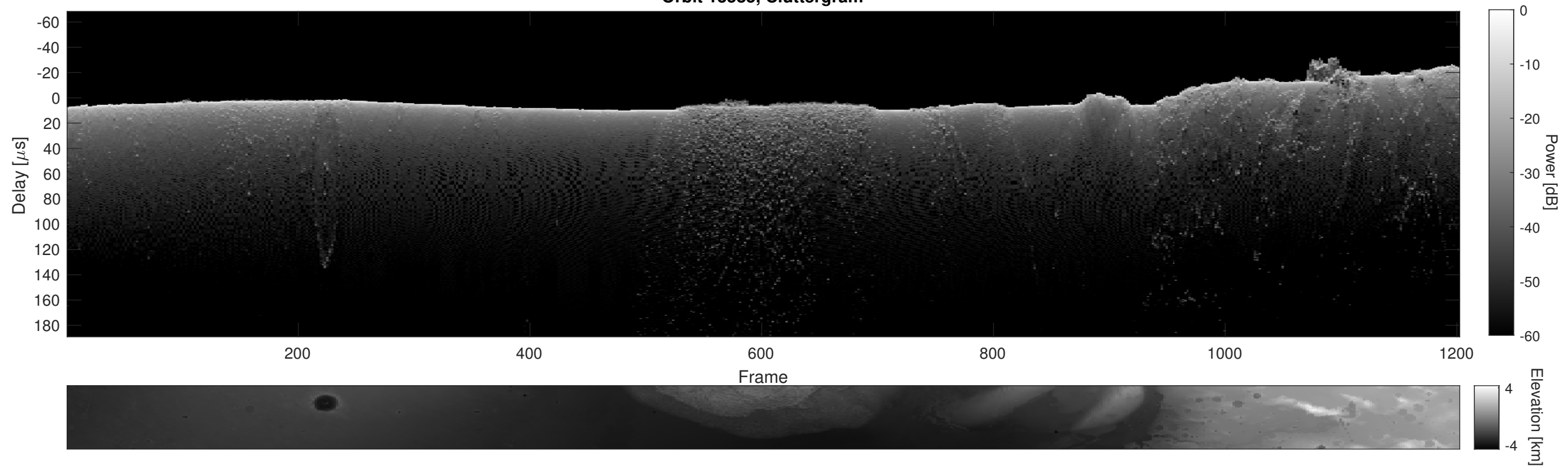
Orbit 13585, Cluttergram
