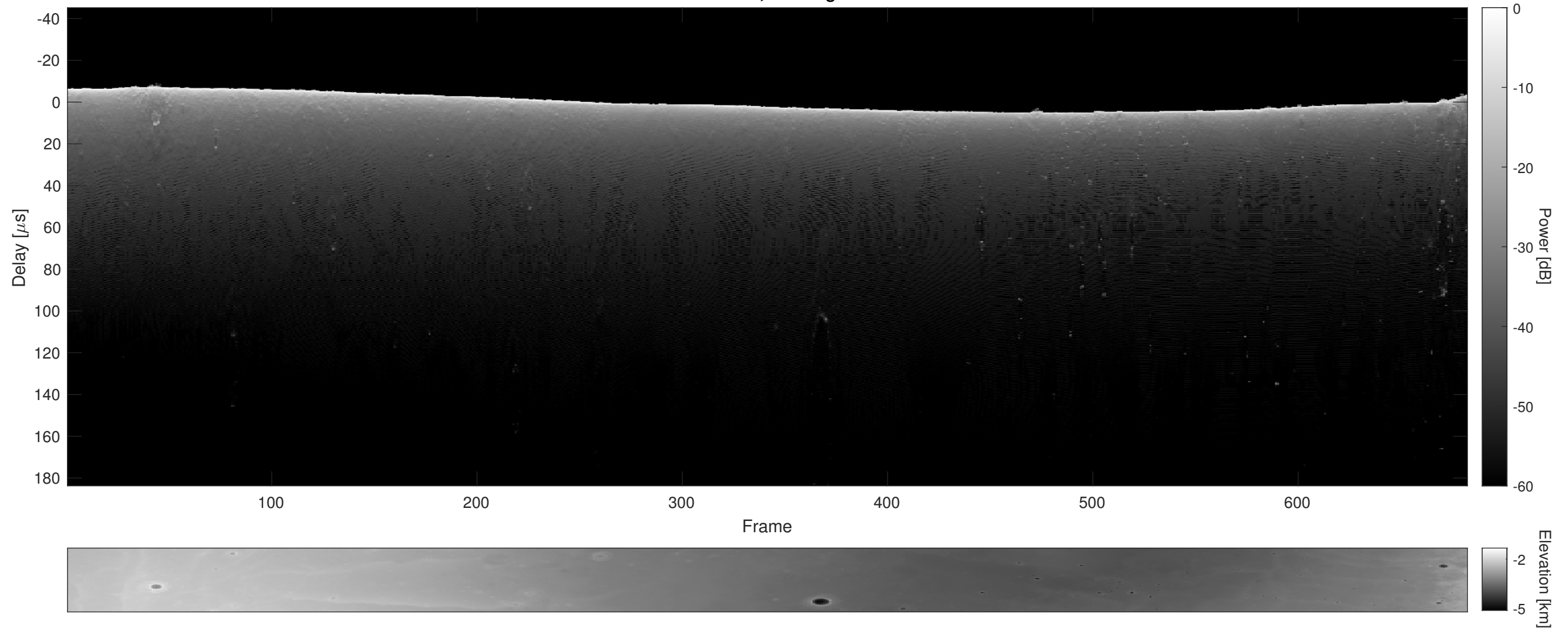
Orbit 13586, Cluttergram
