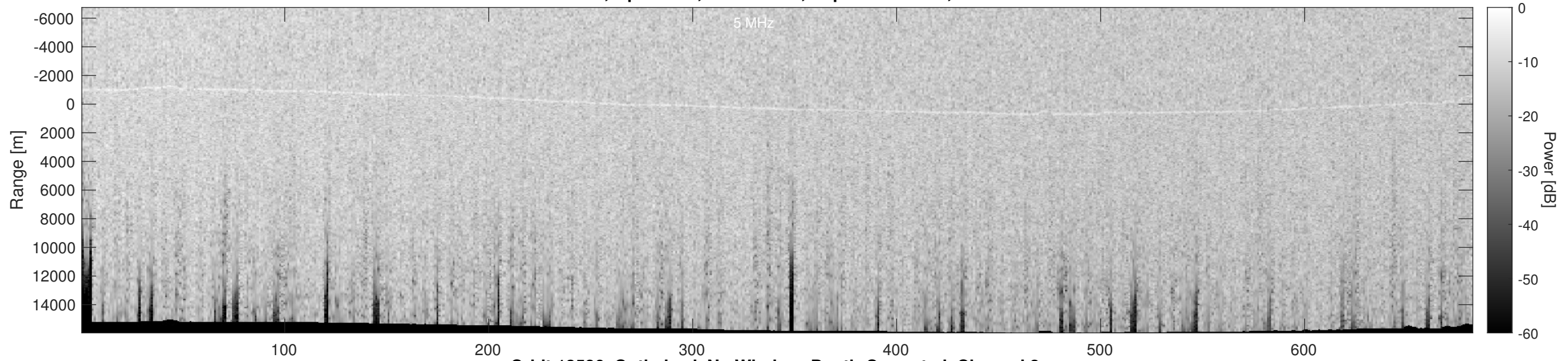
Orbit 13586, Optimized, No Window, Depth-Corrected, Channel 2
