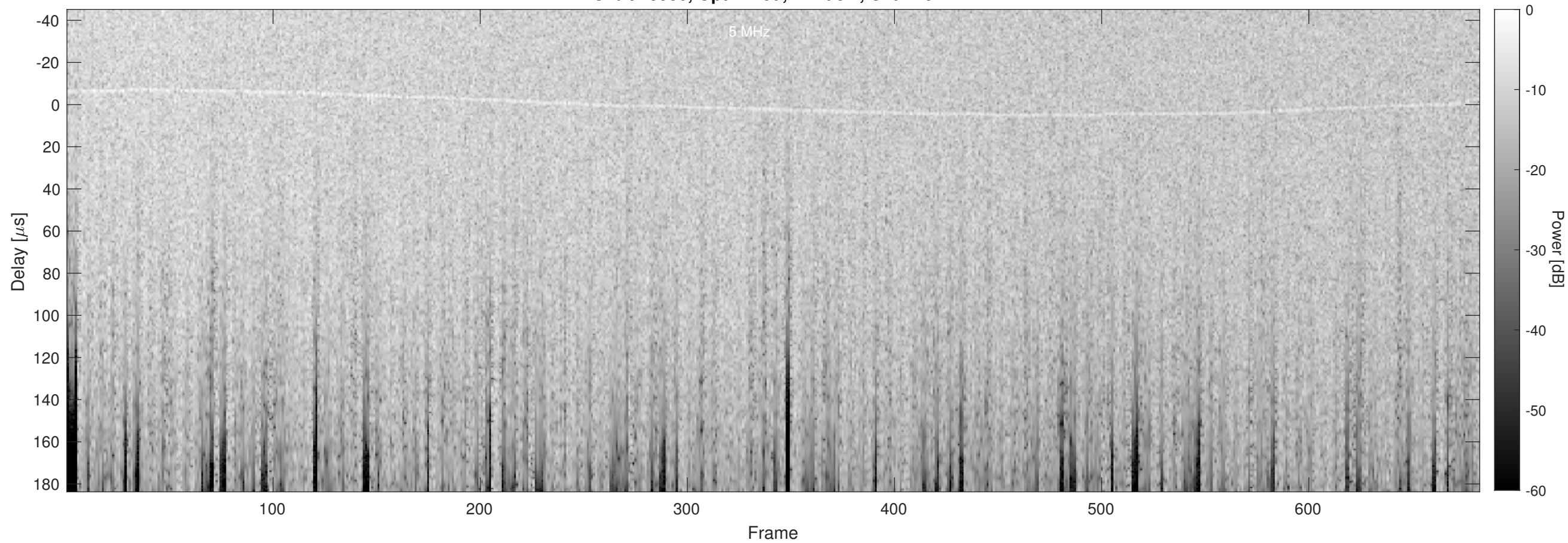
Orbit 13586, Optimized, Window, Channel 2
