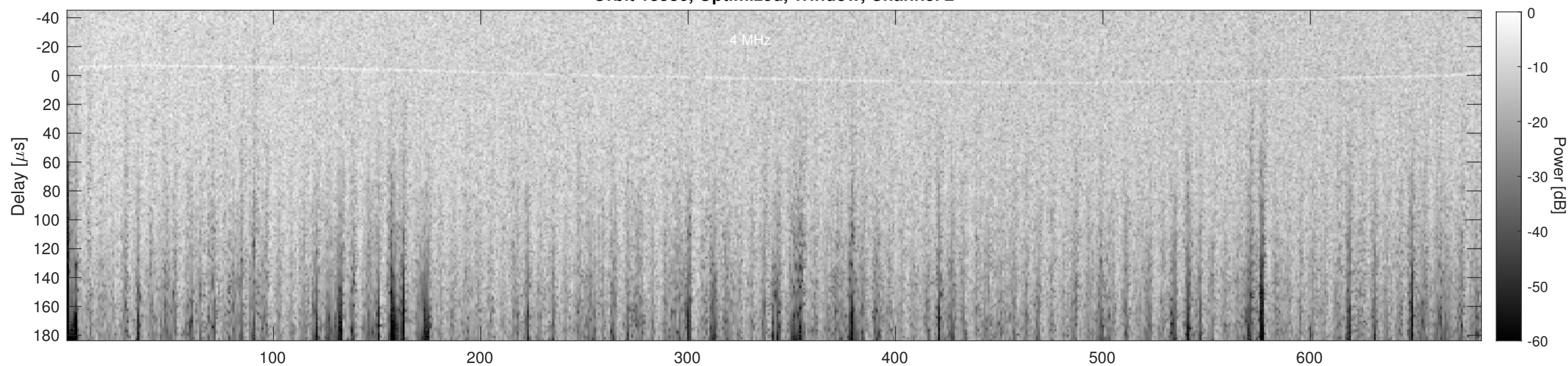
Orbit 13586, Cluttergram
