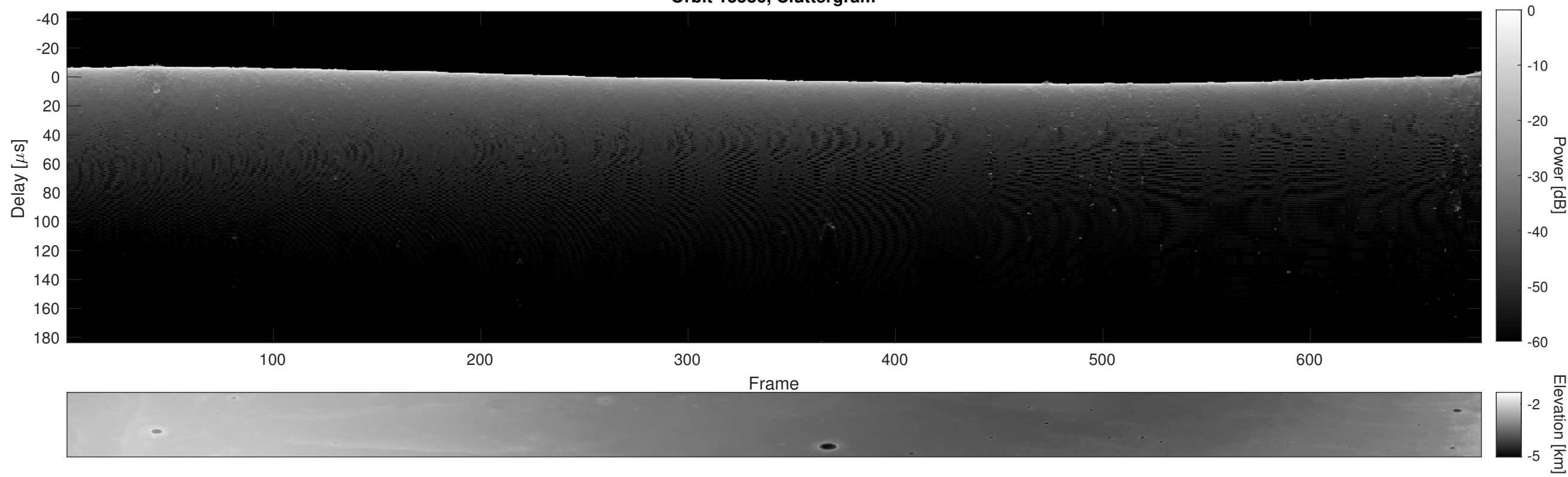
Orbit 13586, Cluttergram
