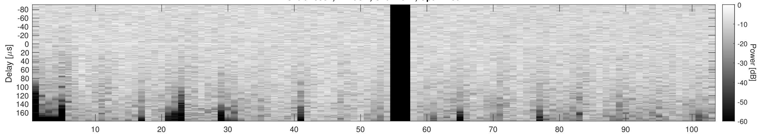
Orbit 13587, Cluttergram
