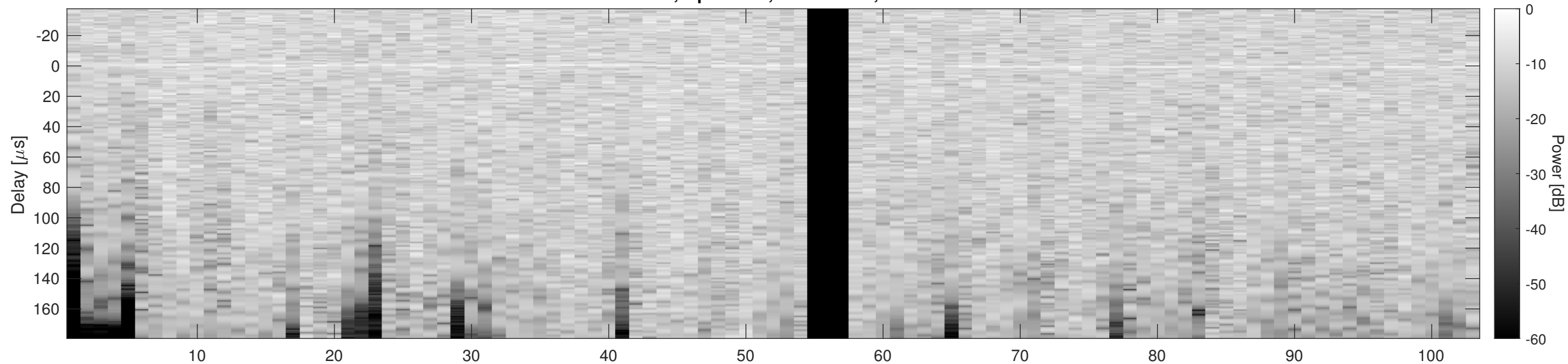
Orbit 13587, Optimized, No Window, Channel 2
