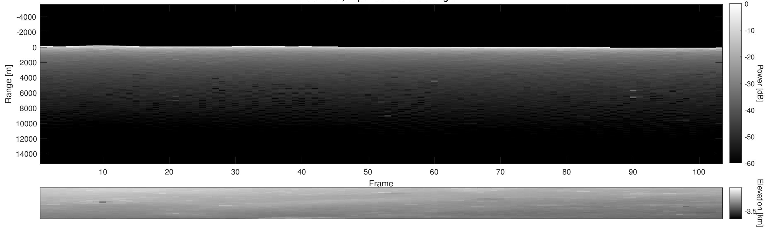
Orbit 13587, Depth-Corrected Cluttergram
