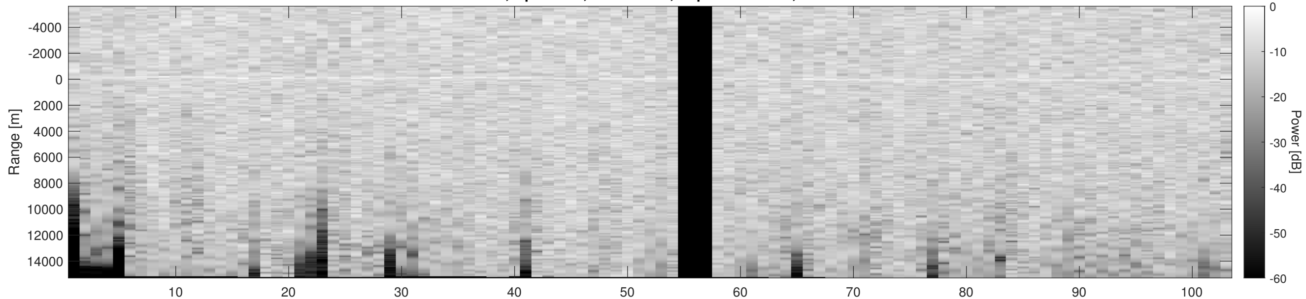
Orbit 13587, Optimized, No Window, Depth-Corrected, Channel 2
