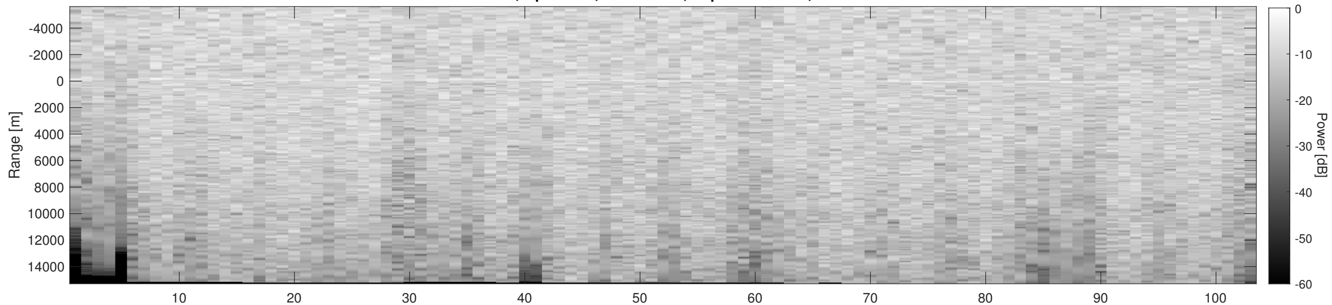
Orbit 13587, Depth-Corrected Cluttergram
