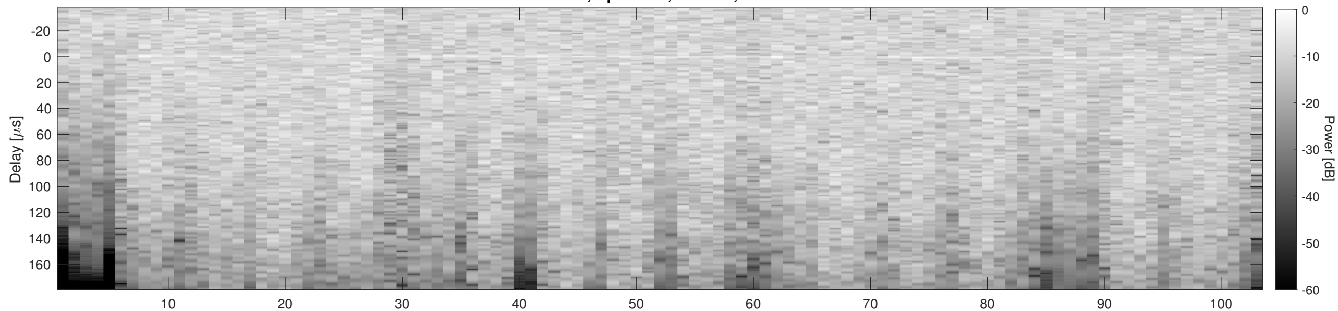
Orbit 13587, Cluttergram
