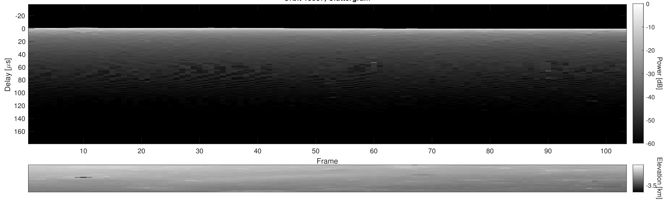
Orbit 13587, Cluttergram
