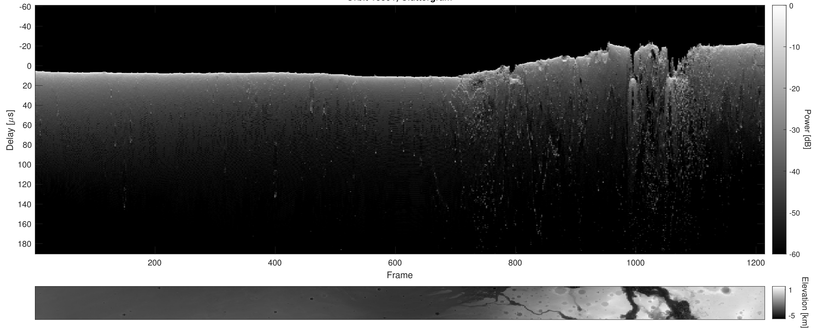
Orbit 13591, Cluttergram
