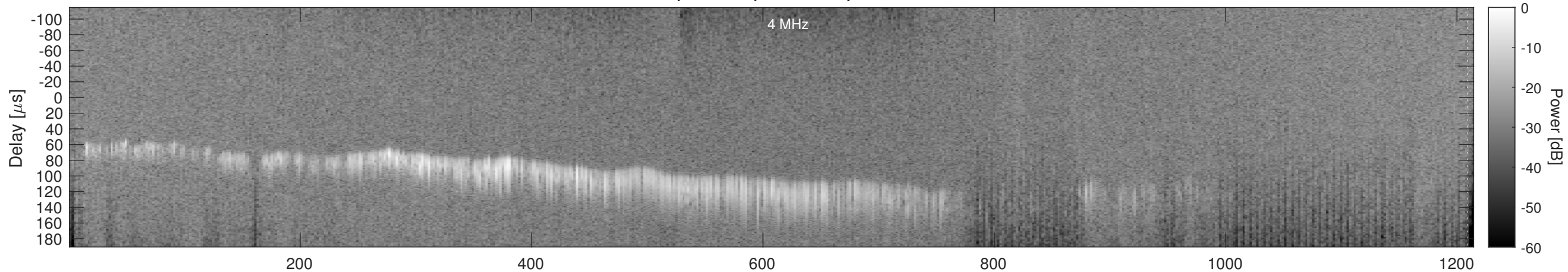
Orbit 13591, Window, Channel 2, Chapman
