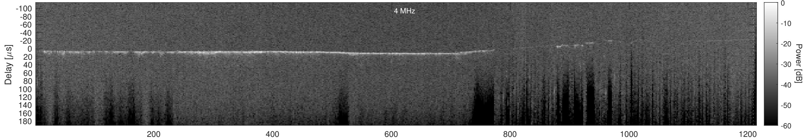
Orbit 13591, Cluttergram
