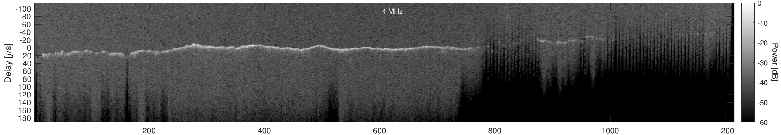
Orbit 13591, Window, Channel 2, Optimized
