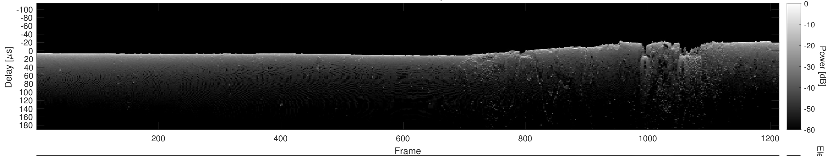
Orbit 13591, Cluttergram
