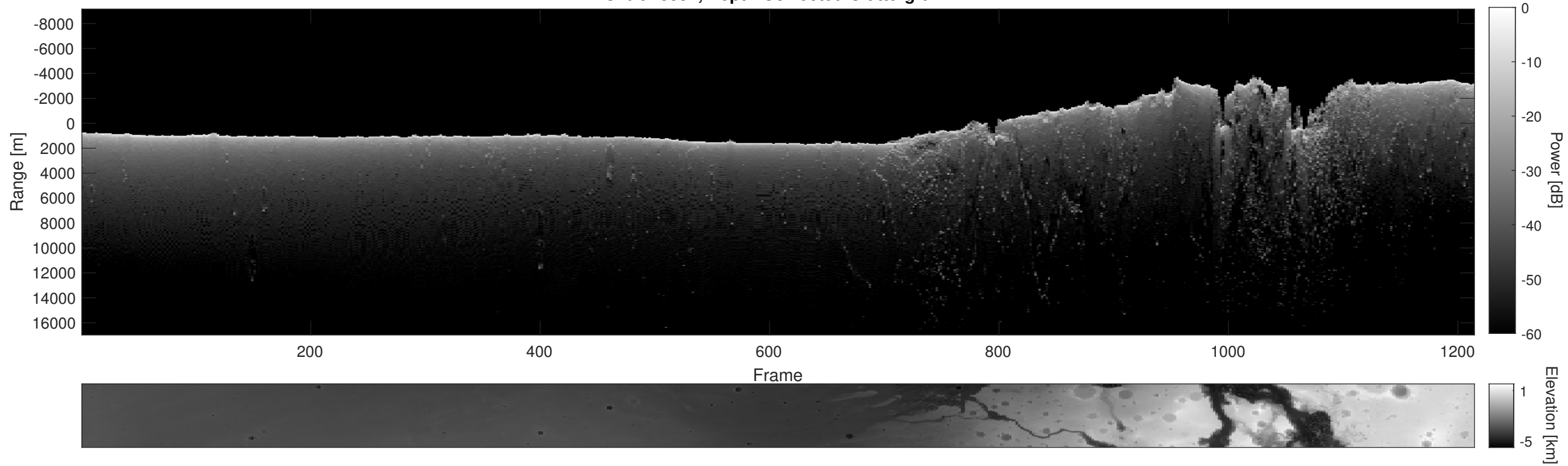
Orbit 13591, Depth-Corrected Cluttergram
