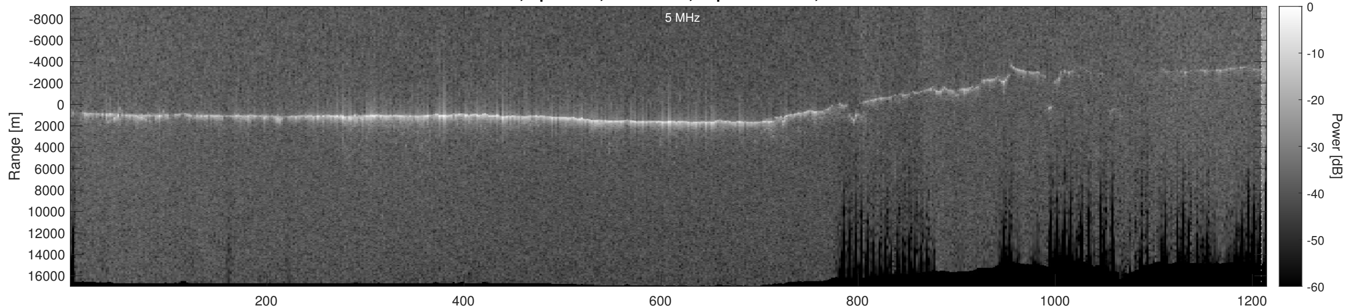
Orbit 13591, Optimized, No Window, Depth-Corrected, Channel 2
