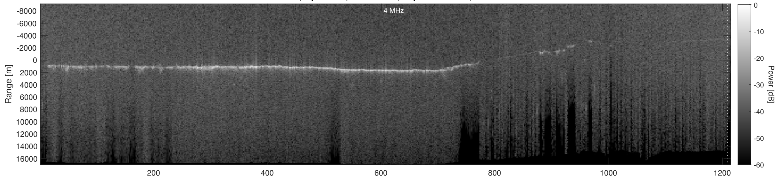
Orbit 13591, Depth-Corrected Cluttergram
