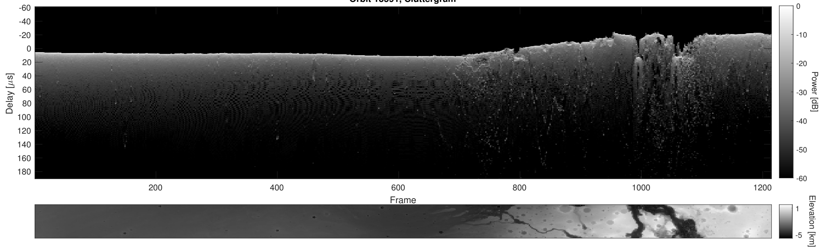
Orbit 13591, Cluttergram
