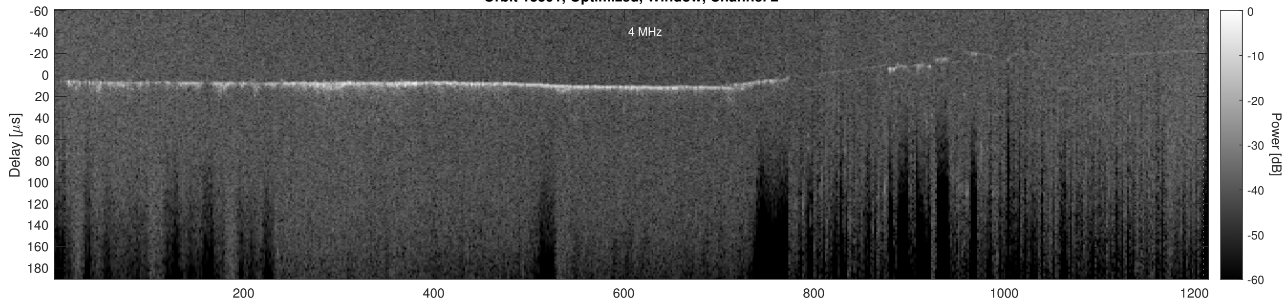
Orbit 13591, Cluttergram
