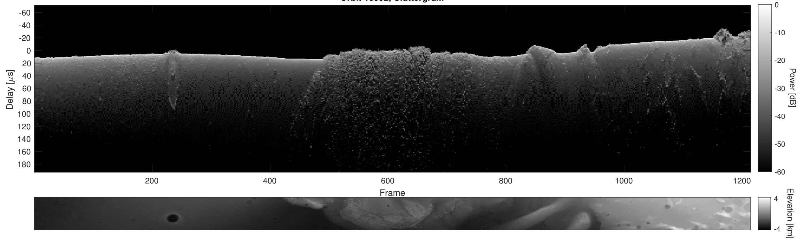
Orbit 13592, Cluttergram
