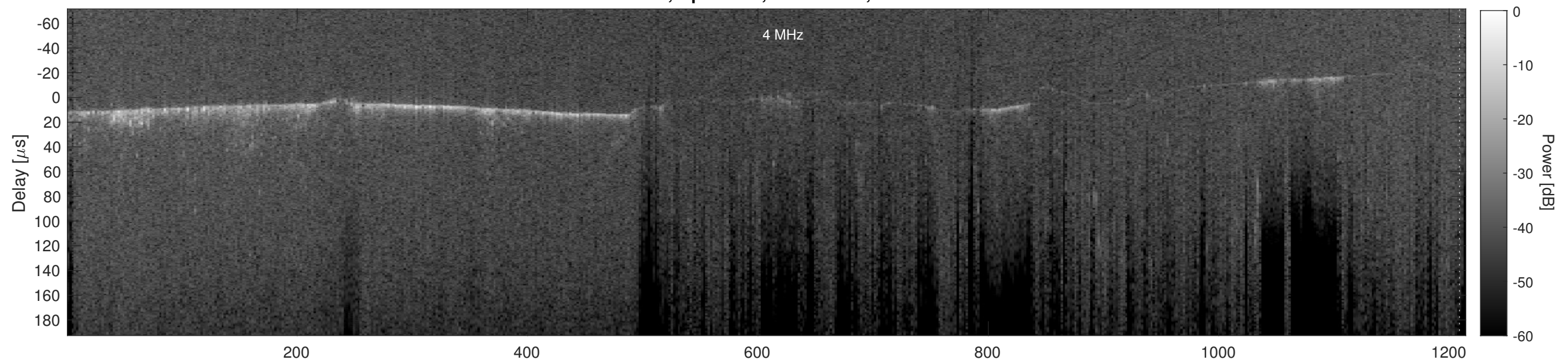
Orbit 13592, Cluttergram
