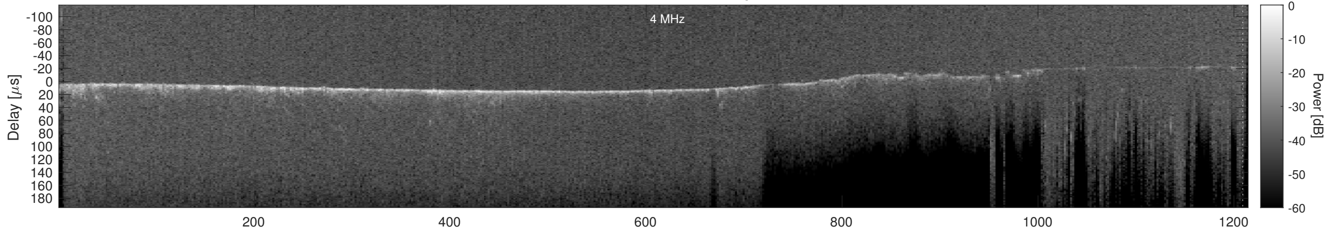
Orbit 13593, Cluttergram
