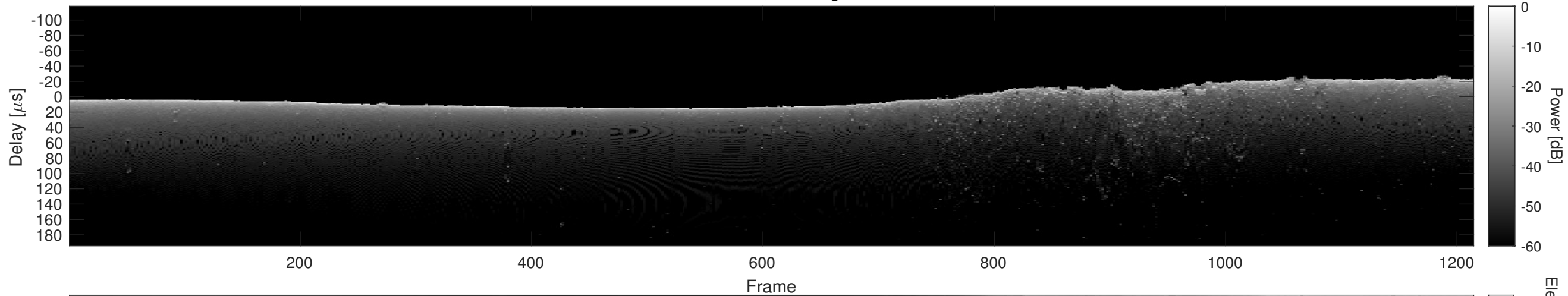
Orbit 13593, Cluttergram
