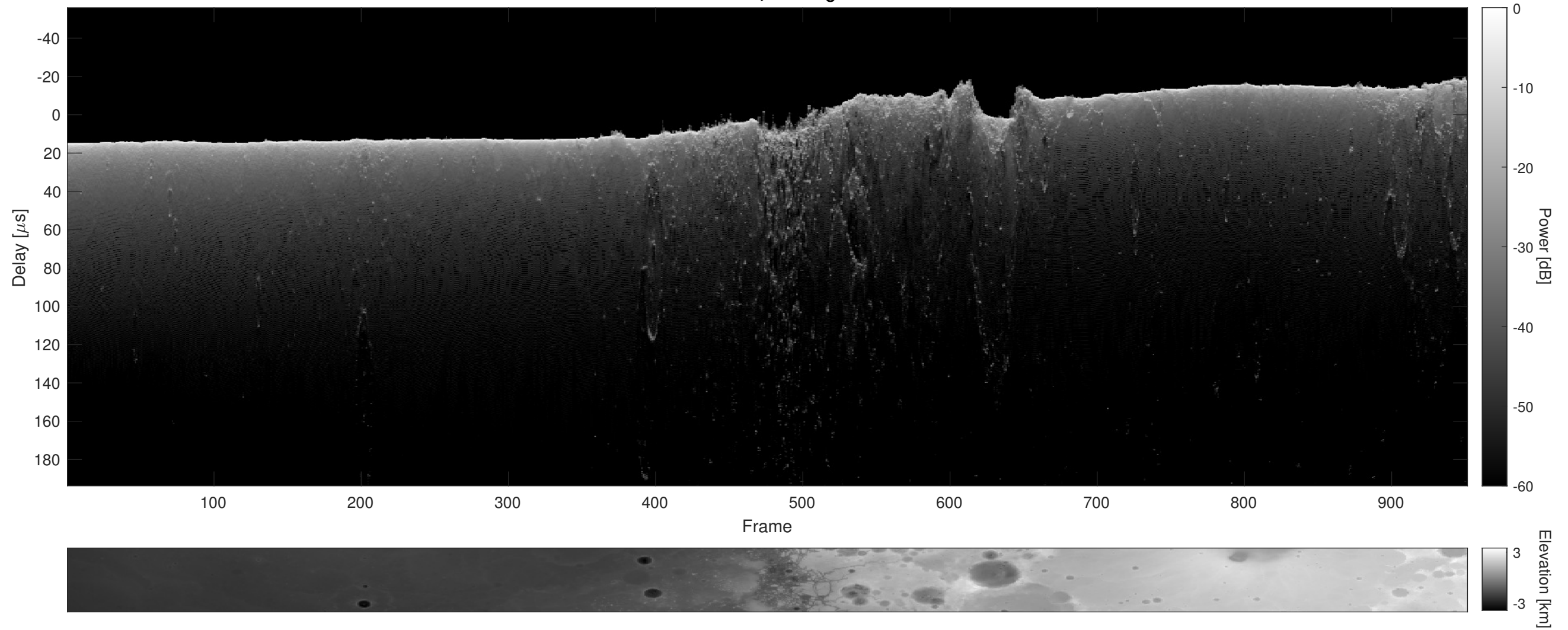
Orbit 13597, Cluttergram
