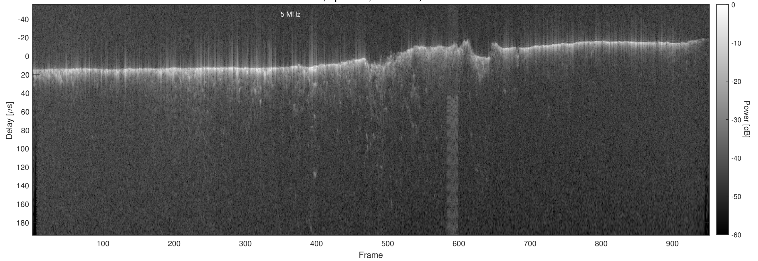
Orbit 13597, Optimized, No Window, Channel 2
