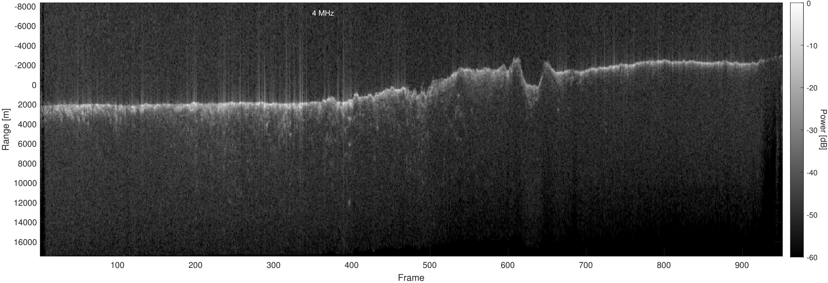
Orbit 13597, Optimized, No Window, Depth-Corrected, Channel 2
