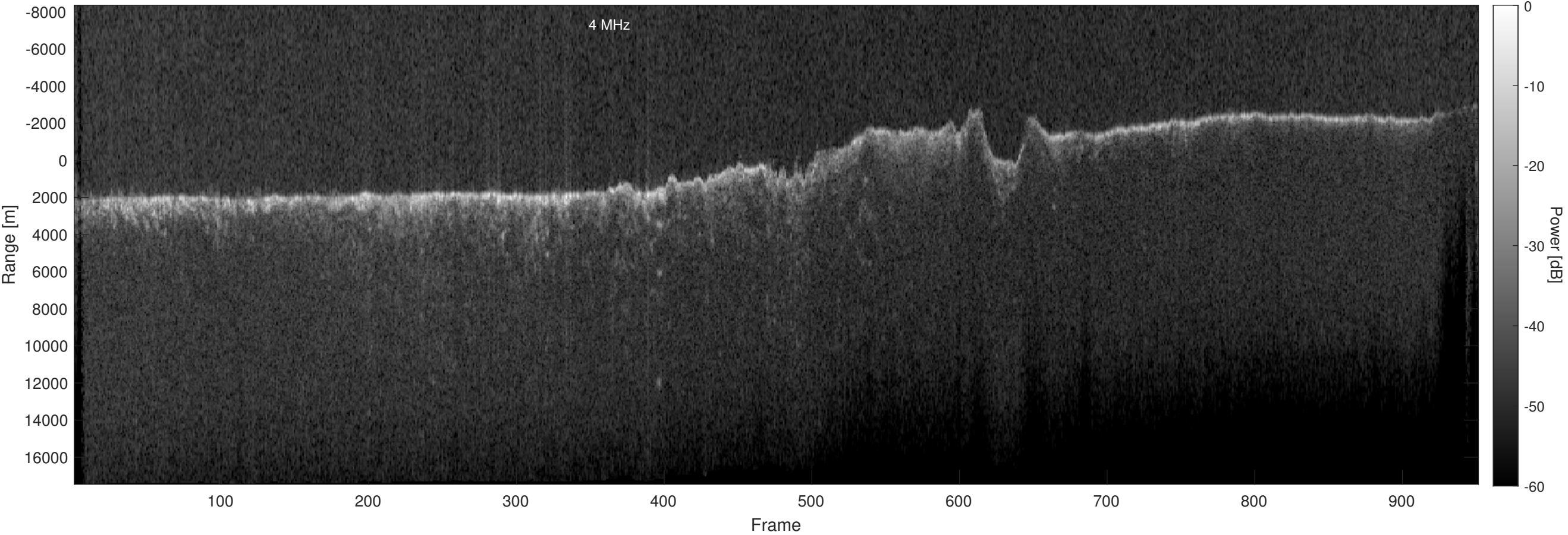
Orbit 13597, Optimized, Window, Depth-Corrected, Channel 2
