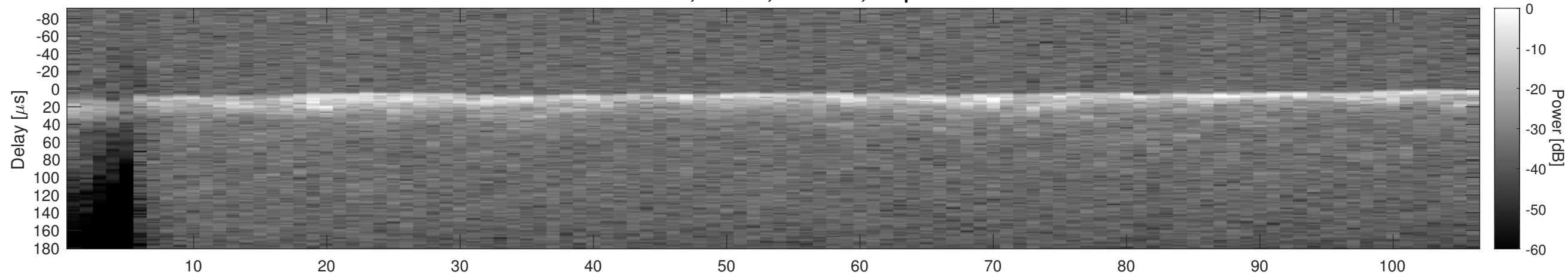
Orbit 13599, Window, Channel 2, Optimized
