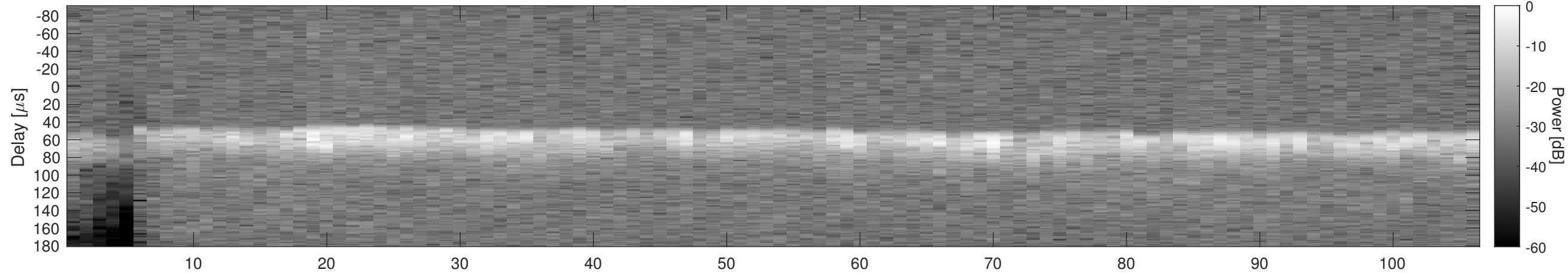
Orbit 13599, Window, Channel 2, Chapman
