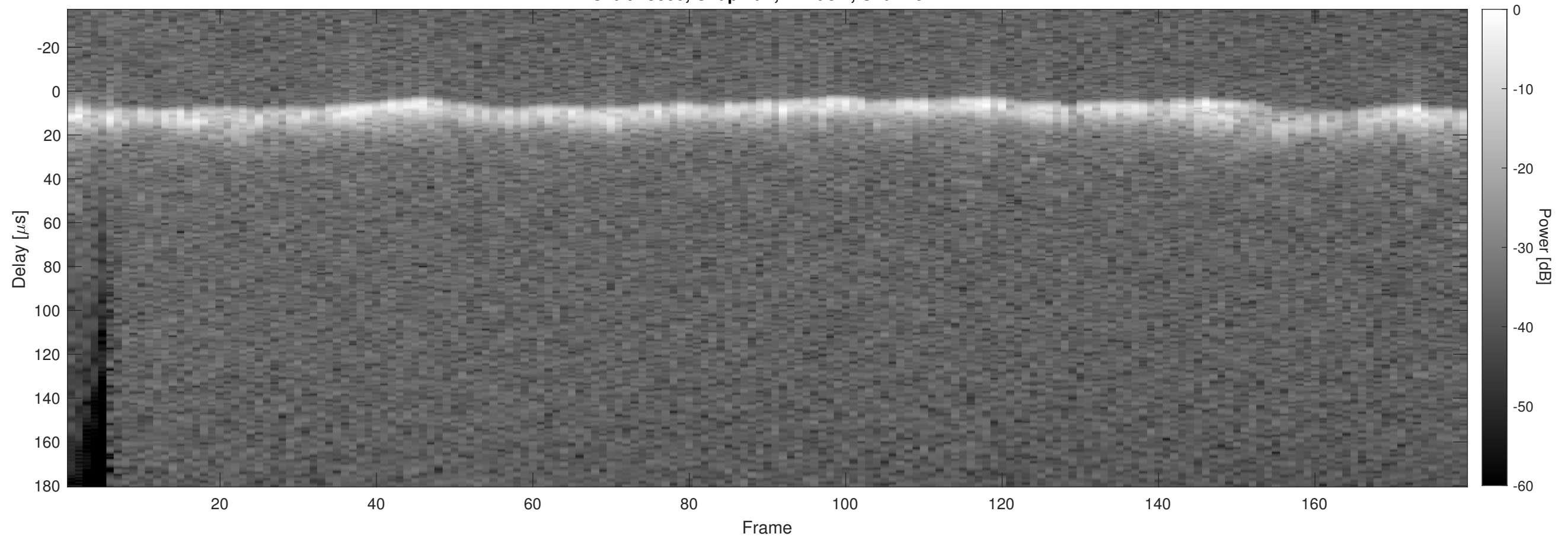
Orbit 13600, Chapman, Window, Channel 2
