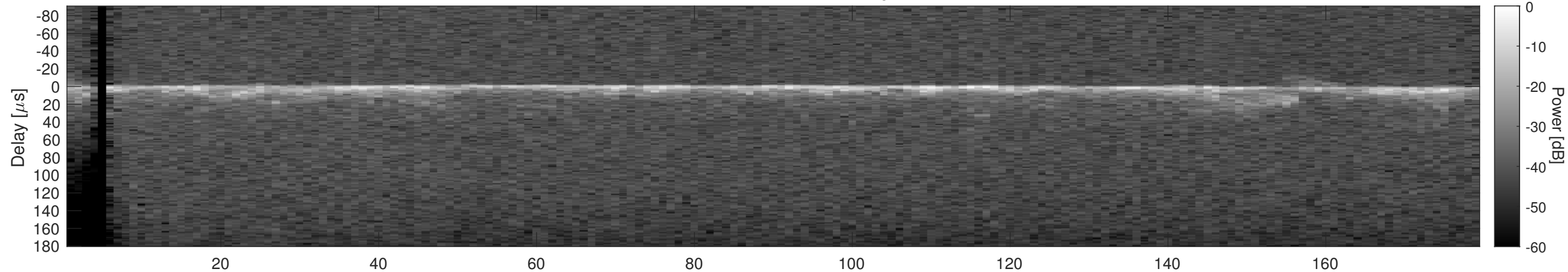
Orbit 13600, Cluttergram
