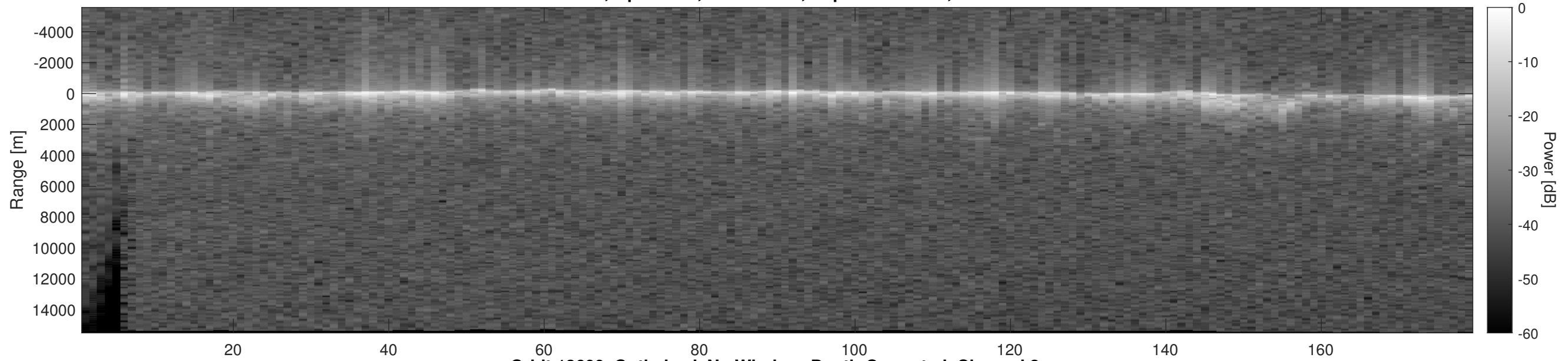
Orbit 13600, Optimized, No Window, Depth-Corrected, Channel 2
