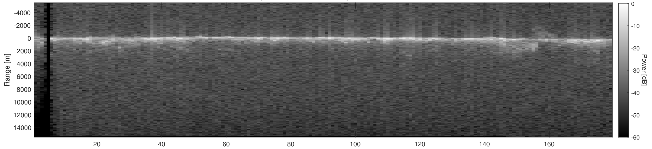
Orbit 13600, Depth-Corrected Cluttergram
