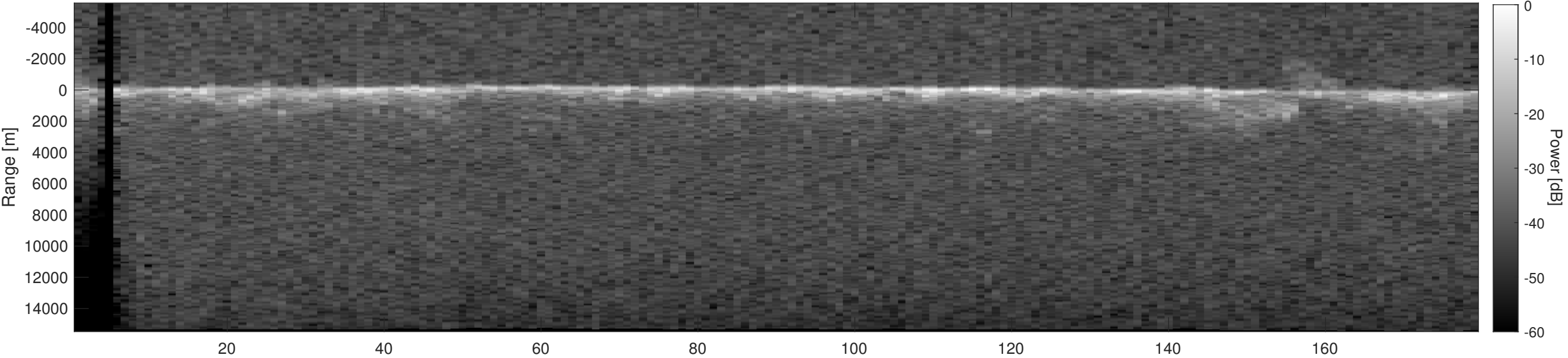
Orbit 13600, Depth-Corrected Cluttergram
