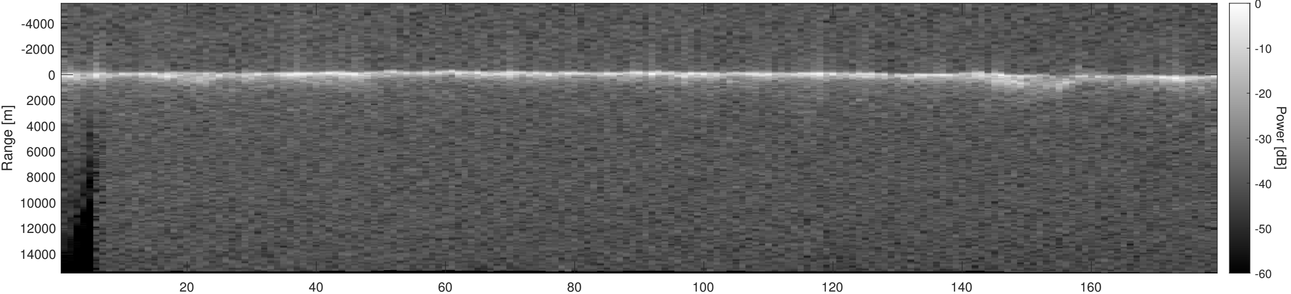
Orbit 13600, Optimized, Window, Depth-Corrected, Channel 2
