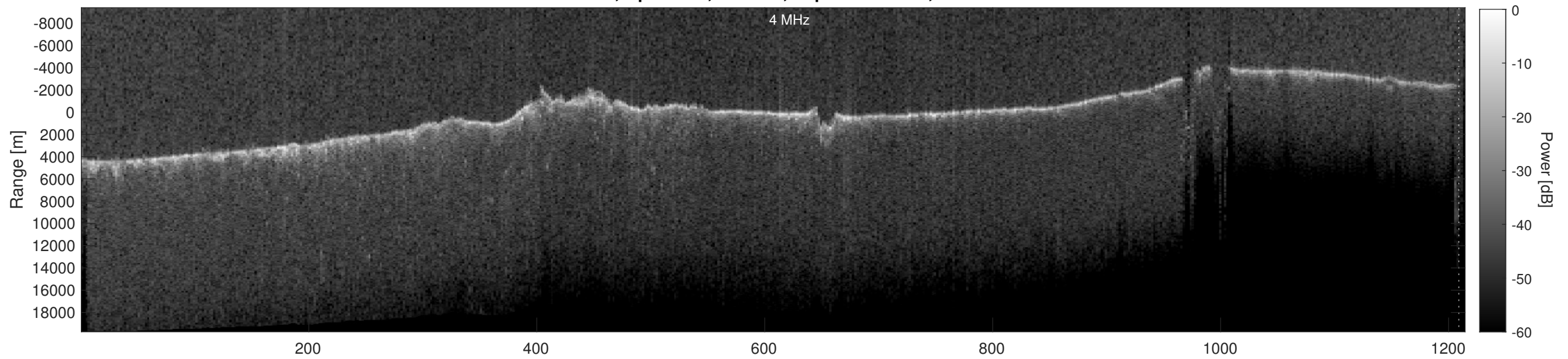
Orbit 13602, Depth-Corrected Cluttergram
