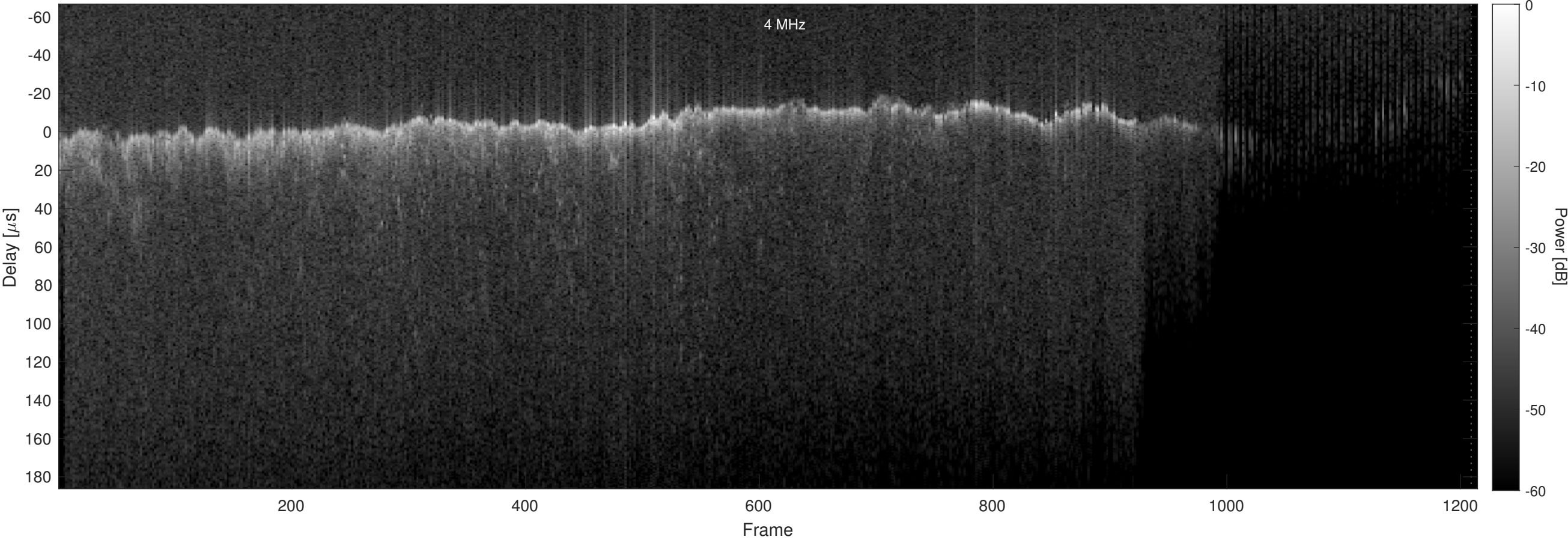
Orbit 13603, Chapman, No Window, Channel 2
