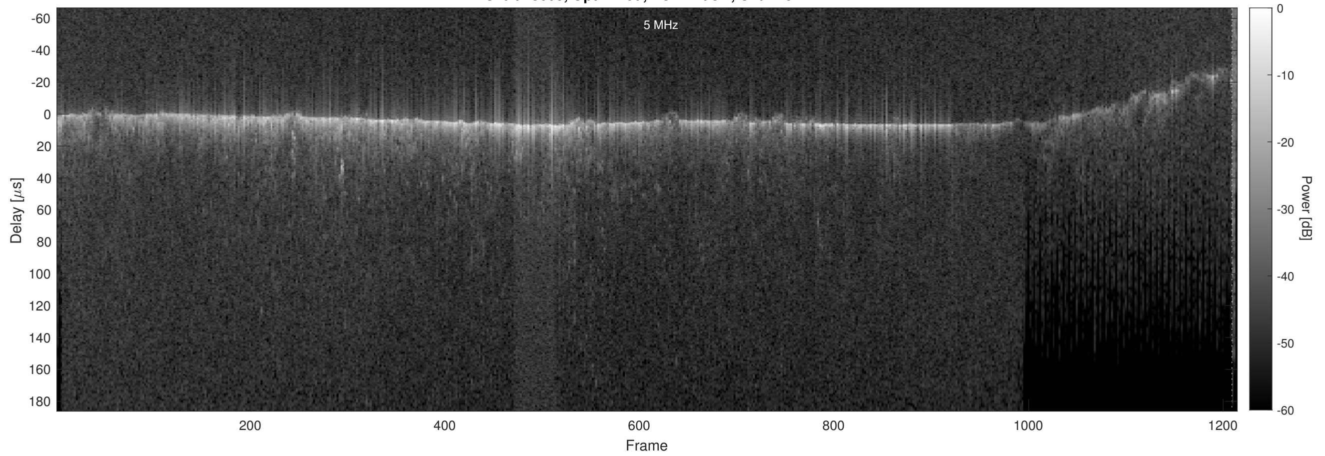
Orbit 13603, Optimized, No Window, Channel 2
