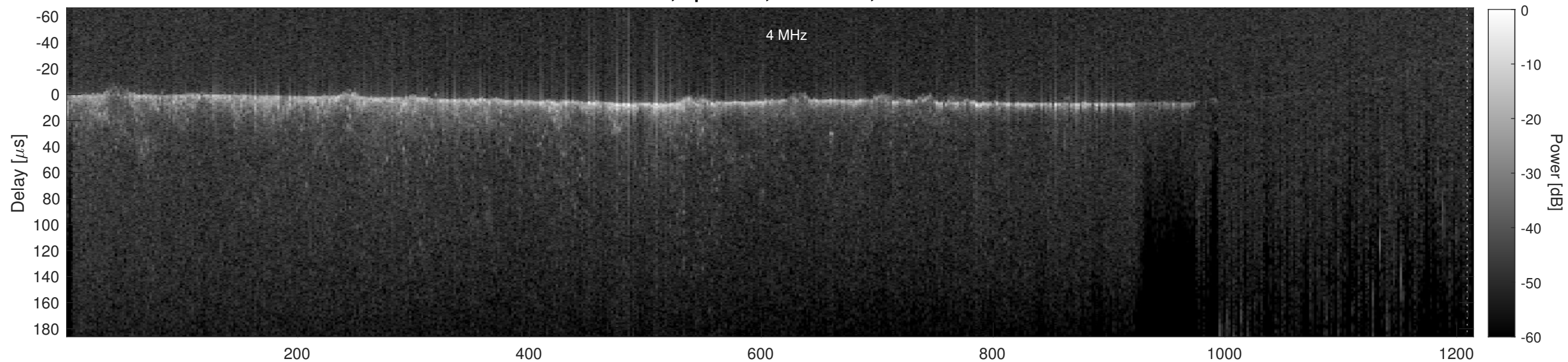
Orbit 13603, Cluttergram
