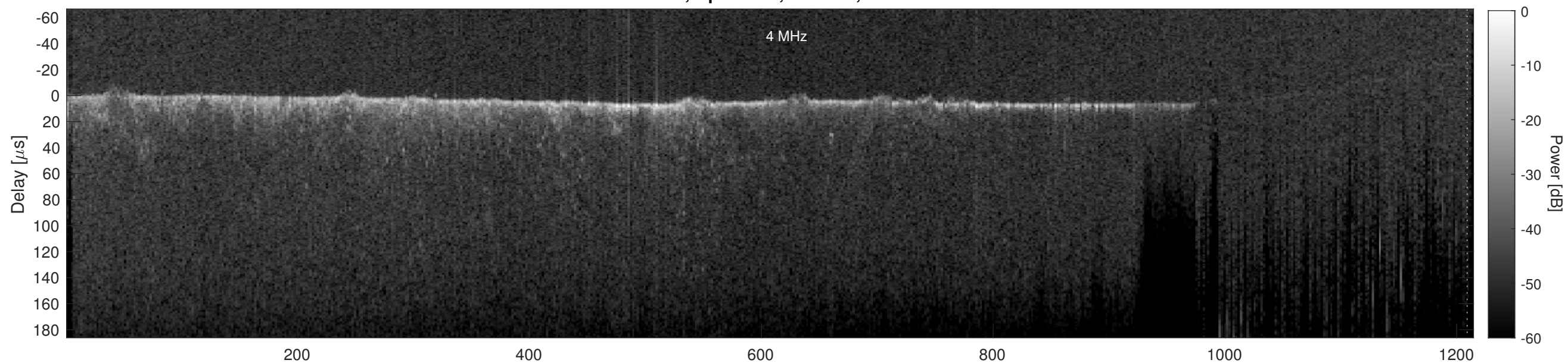
Orbit 13603, Cluttergram
