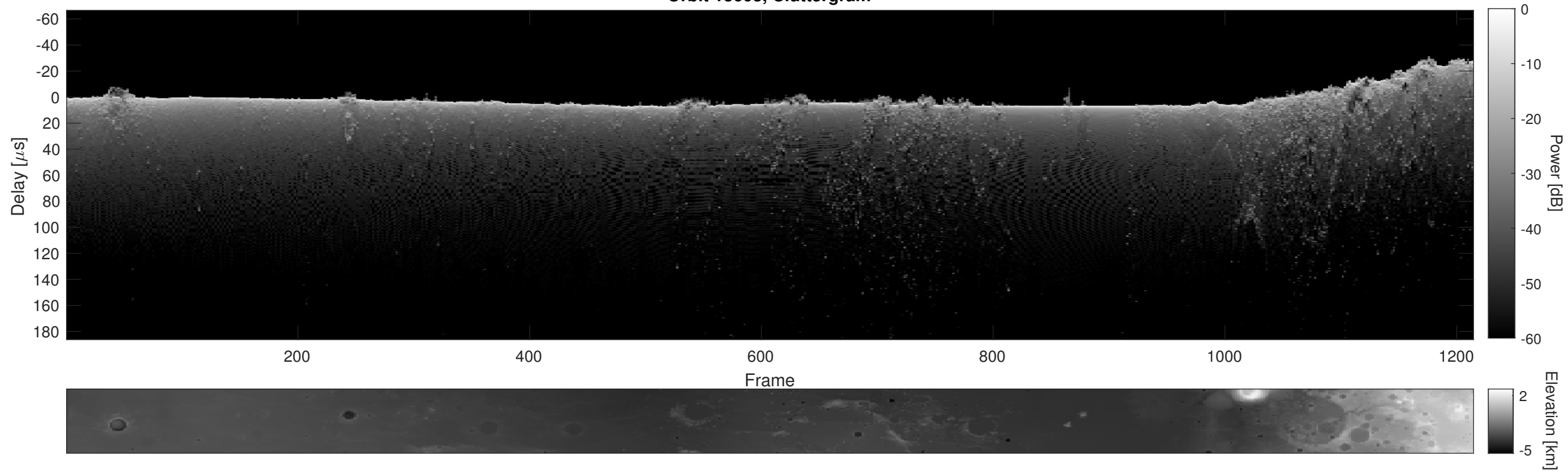
Orbit 13603, Cluttergram
