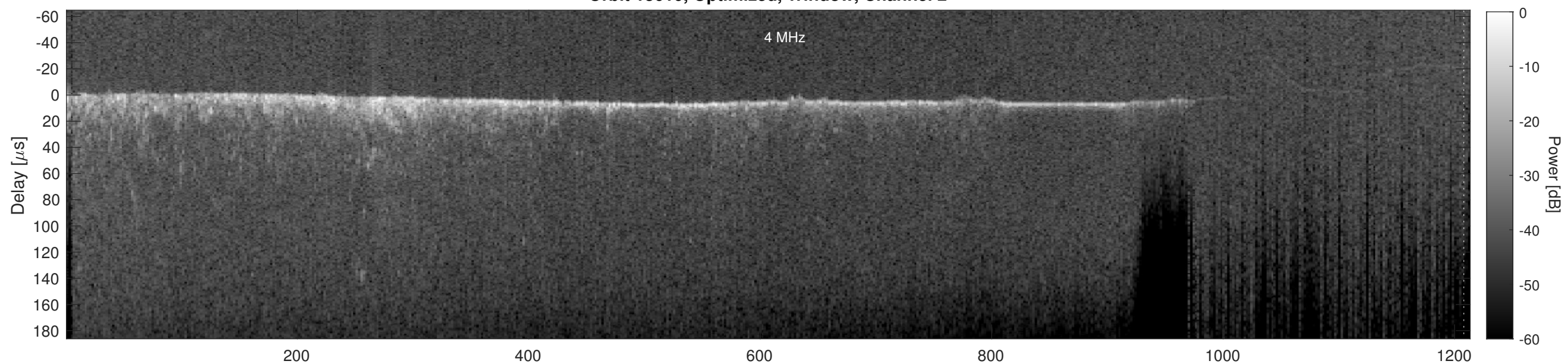
Orbit 13610, Cluttergram
