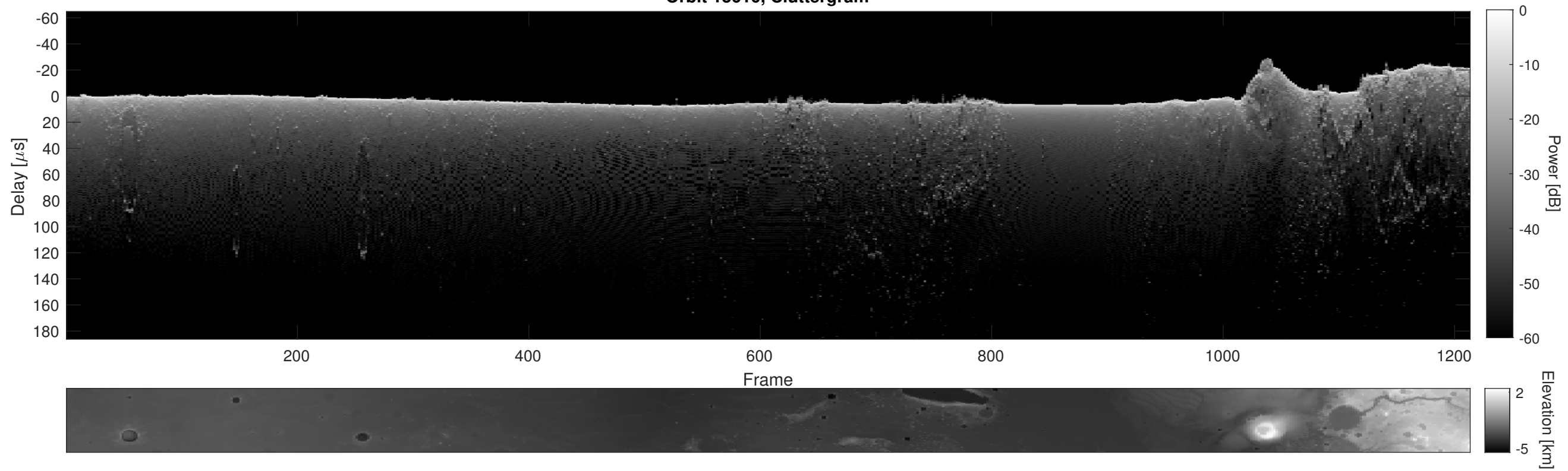
Orbit 13610, Cluttergram
