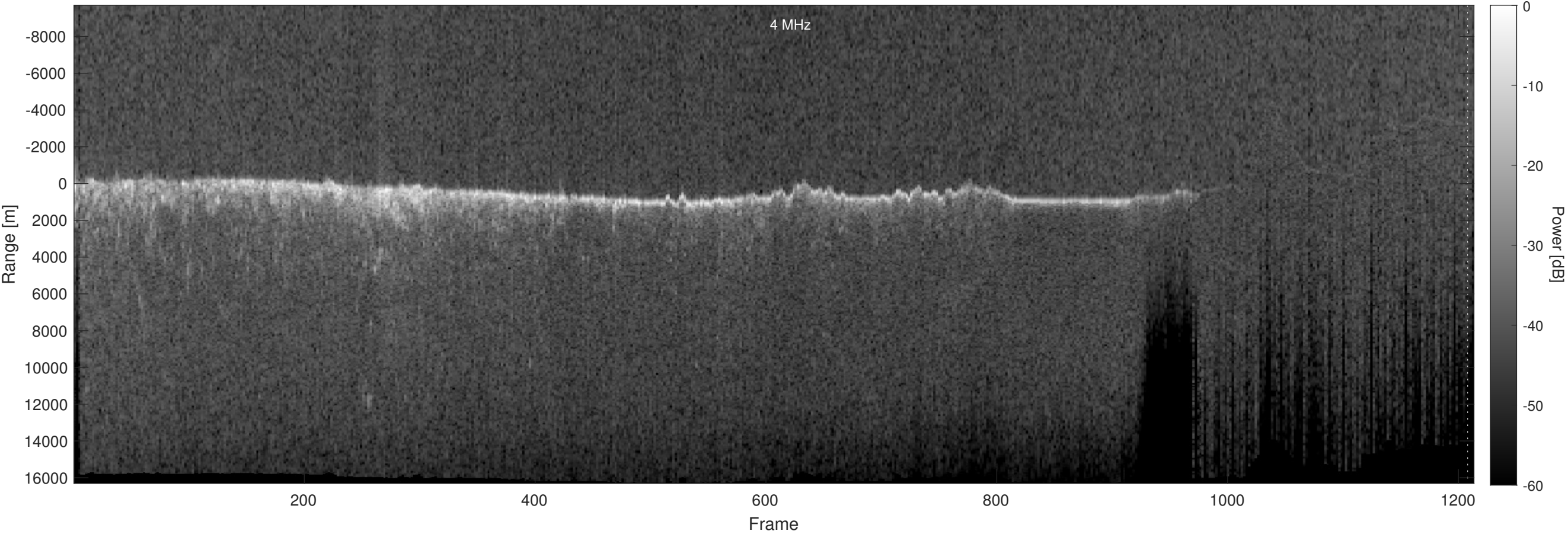
Orbit 13610, Optimized, Window, Depth-Corrected, Channel 2
