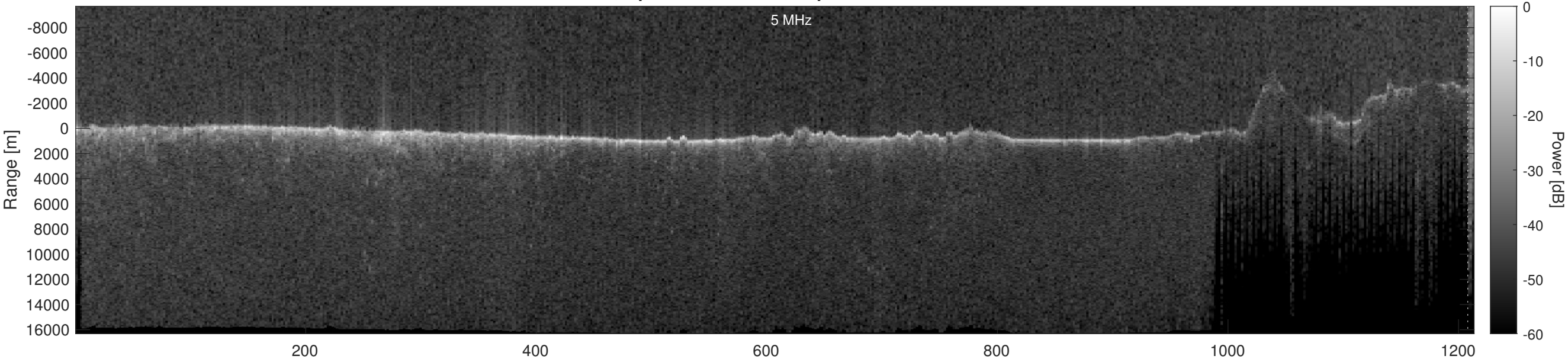
Orbit 13610, Optimized, Window, Depth-Corrected, Channel 2
