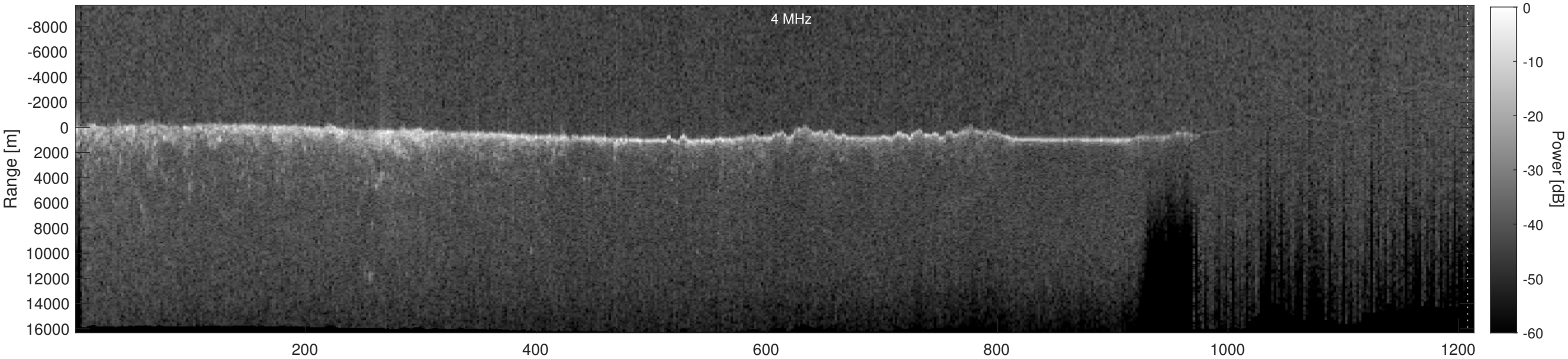
Orbit 13610, Depth-Corrected Cluttergram
